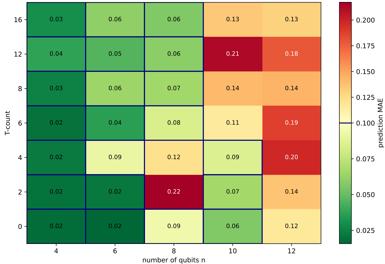
Algorithm 1 hardness diagram (N = 5000, depth = 3, 2 instances per cell)
