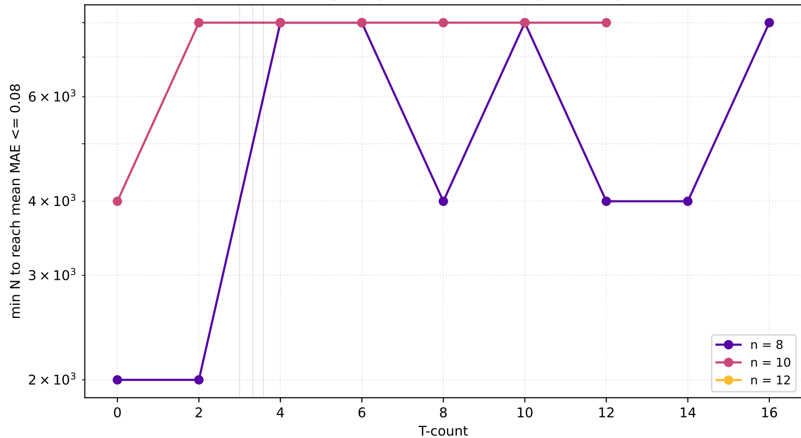
T-count hardness boundary (depth=3, 3 instances per cell, eps=0.3, tau=0.05)
