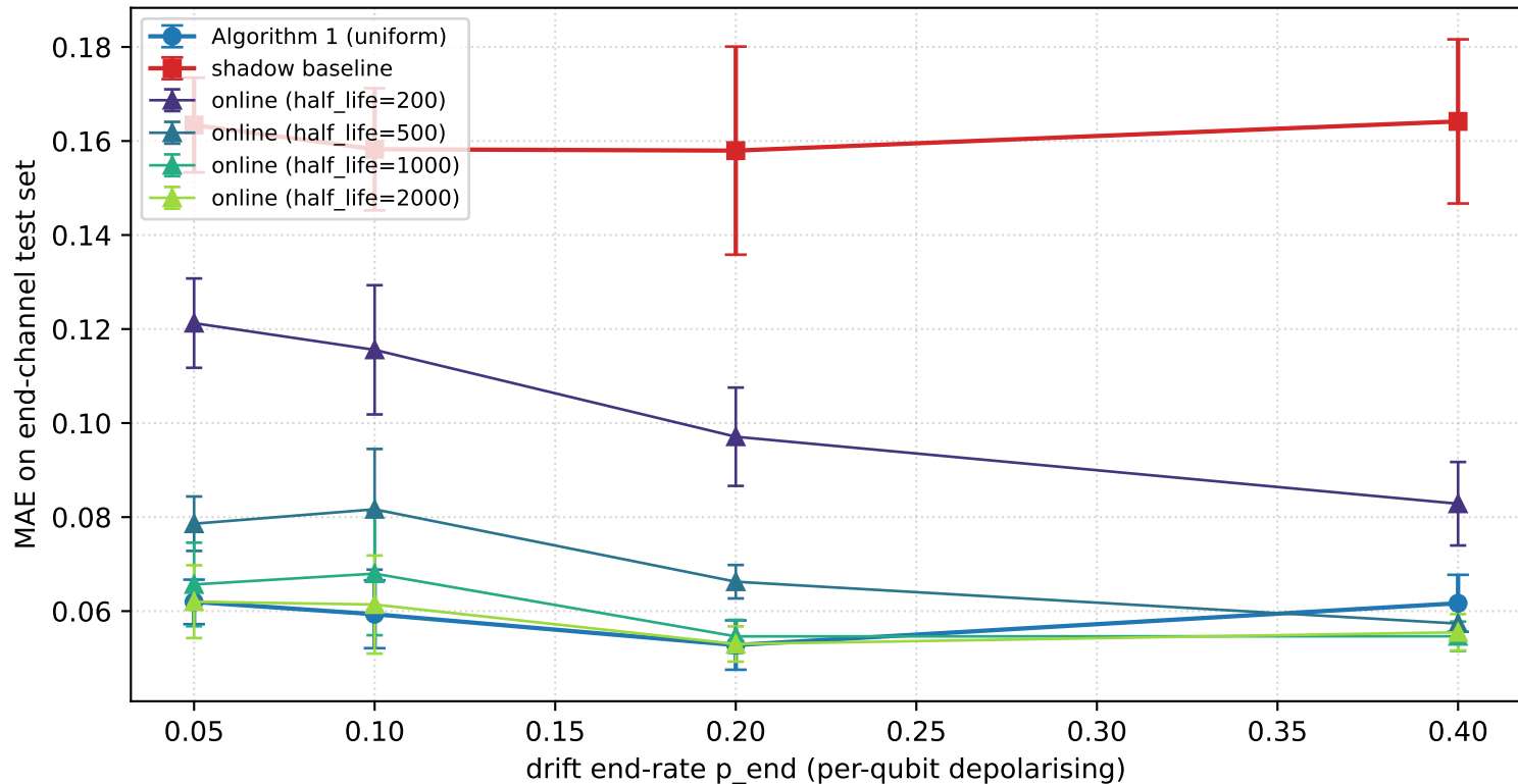
Drift-aware Algorithm 1 ( n=4 , N=4000 , 4 instances)
