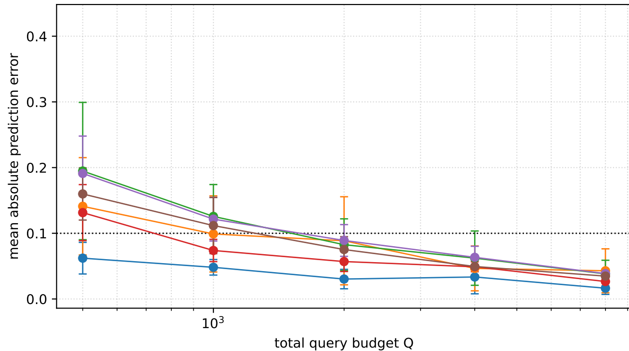
QPSQ (Algorithm 1)
