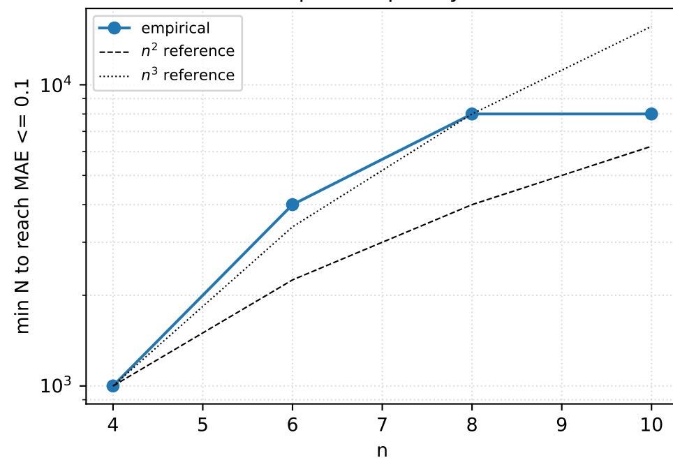
Sample complexity vs n
