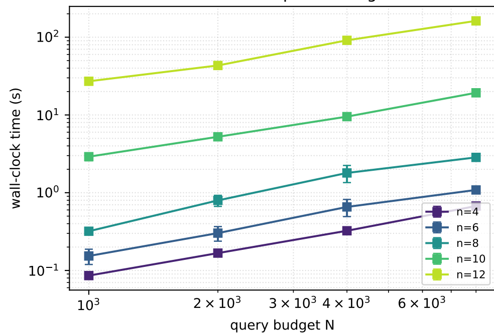
Wall-clock time per training run
