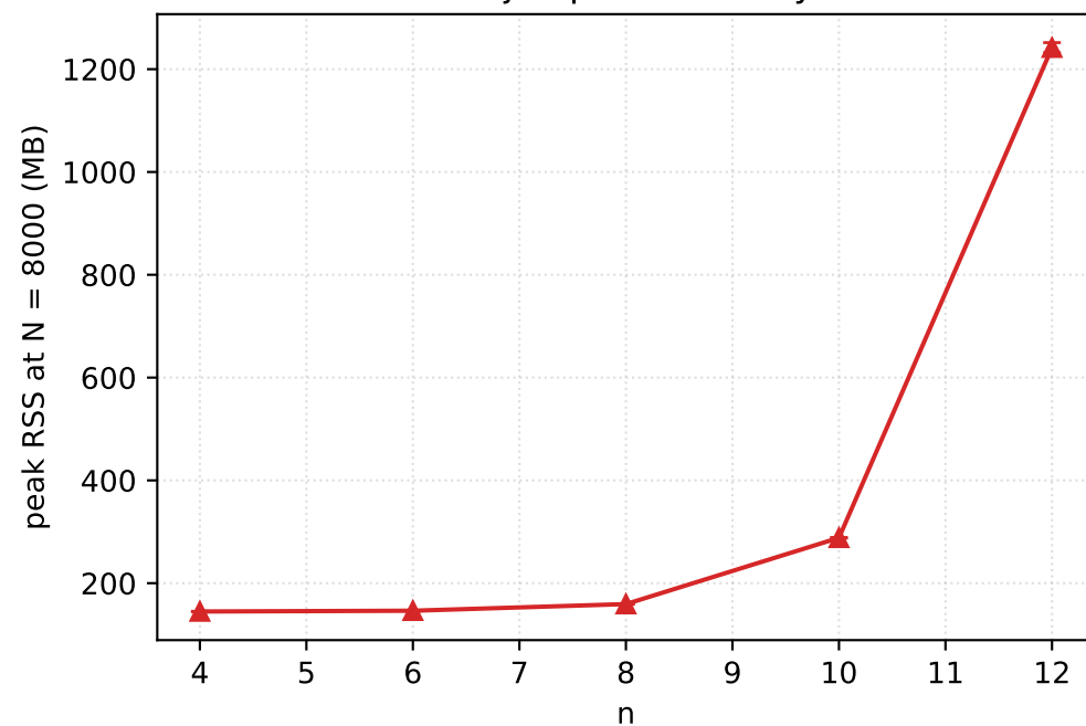
Per-job peak memory
