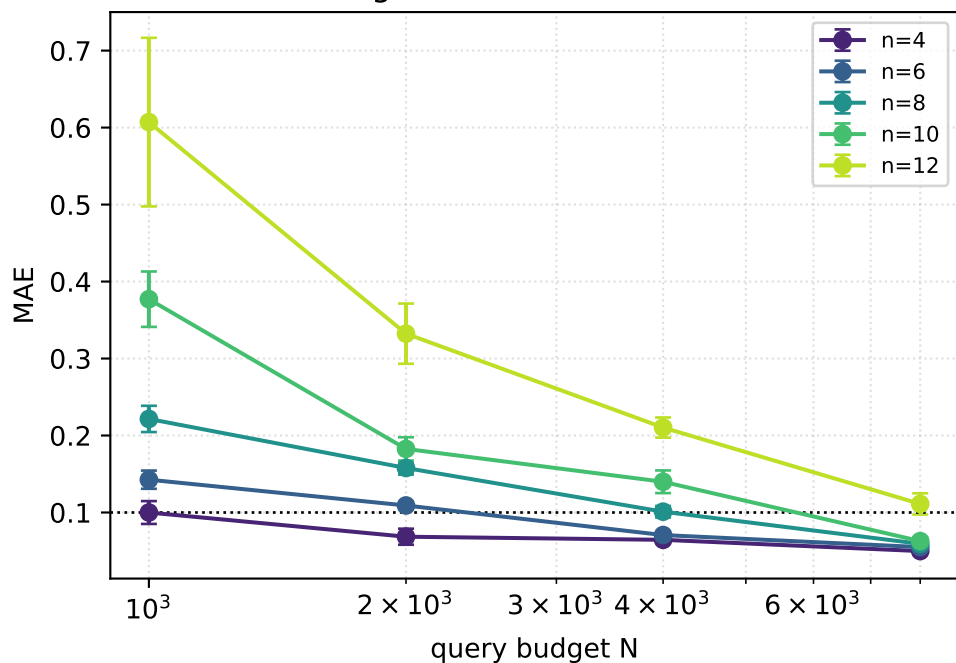
Convergence: MAE vs N for each n
