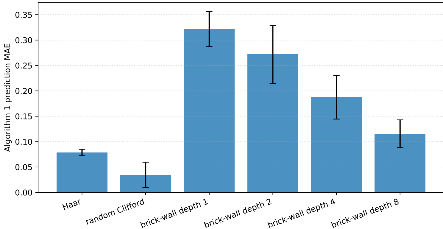
Prediction MAE across unitary ensembles ( n=6 , \tau=0.05 , N=4000 , 8 instances each)
