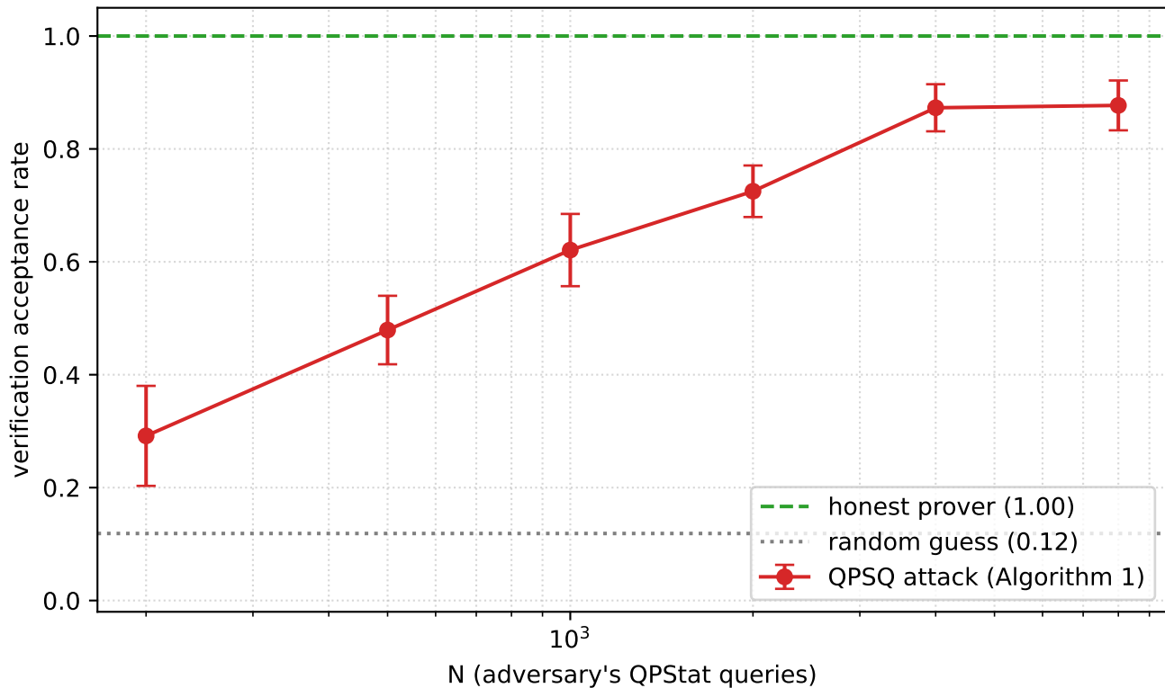
CR-QPUF attack via Algorithm 1 ( n=4 , threshold=0.1, 6 devices)
