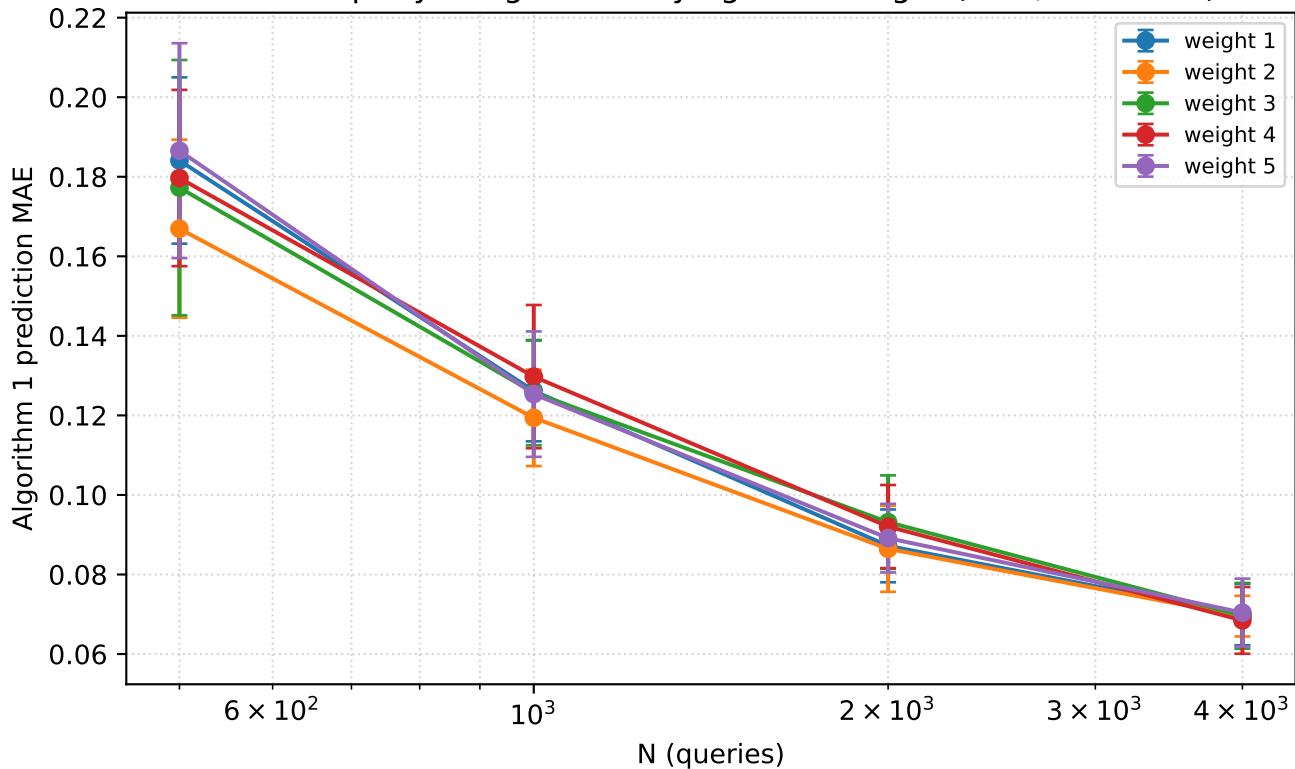
MAE vs. query budget for varying Pauli weight (n=5, tau=0.05)
