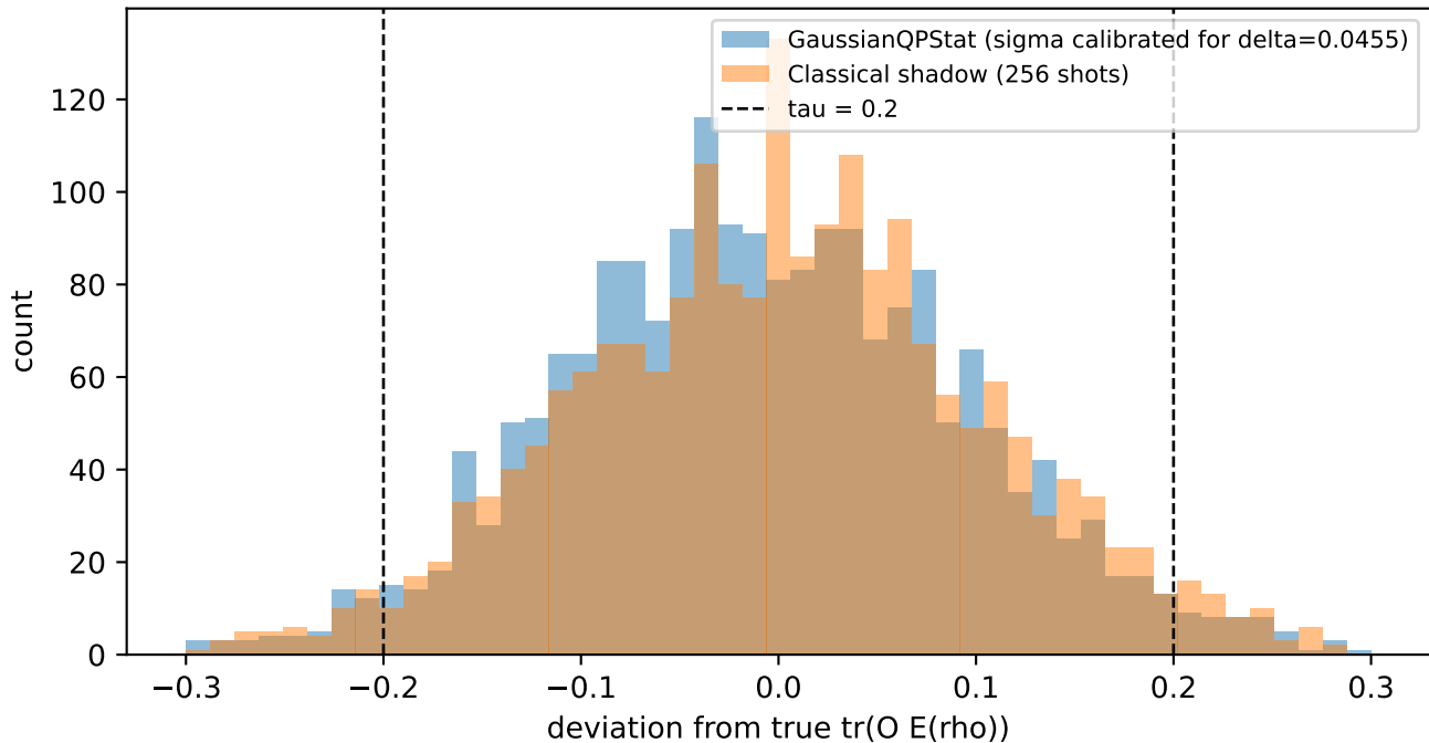
Fig. 1 reproduction (n=1 fixed Haar U, O=Z, 2000 stab states)
