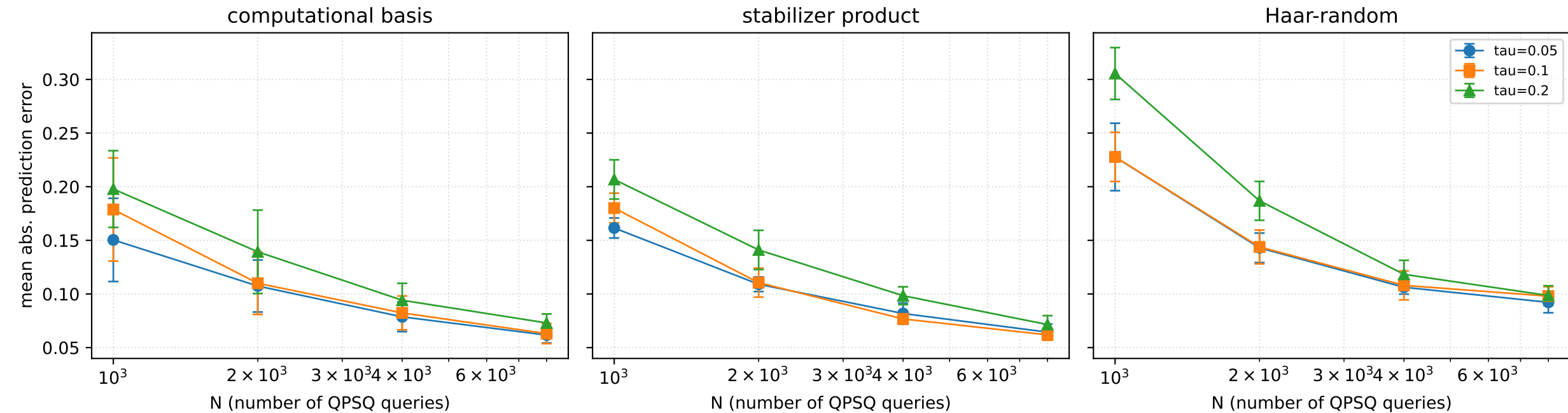
Fig. 2 reproduction (n=6, eps=0.3, 10 Haar unitaries, observable Z_0)
