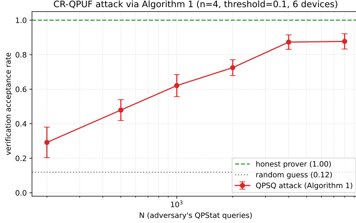
Figure 6: The QPSQ adversary’s acceptance rate climbs from \sim 29\% at N = 200 to \sim 88\% at N = 4,000 , well above the \sim 12\% random-guess baseline and approaching the honest prover’s 100%. This is a small-scale empirical validation of the paper’s quasipolynomial attack.
