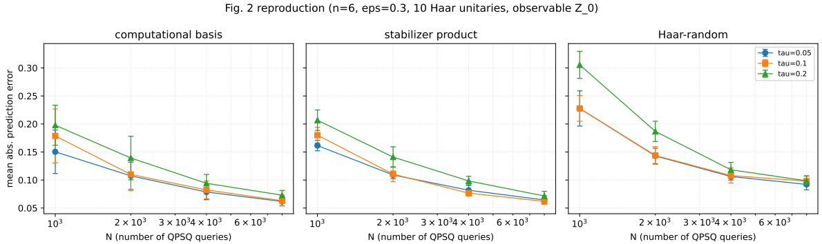
Figure 2: Reproduction of paper Figure 2. Mean absolute prediction error vs. number of QPSQ queries N for Algorithm 1 on 10 Haar-random 6-qubit unitaries with observable O = Z_0 , target prediction error \epsilon = 0.3 , and three QPStat tolerances. Three panels correspond to three target-state trends. Lower \tau and larger N both reduce error, matching the paper’s qualitative trends.
