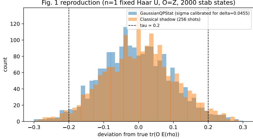
Figure 1: Reproduction of paper Figure 1. Both methods stay within the stated tolerance in \sim 95\% of trials, matching 1 - \delta . The Gaussian emulator is calibrated to saturate this bound while shadows with 256 shots achieve a comparable empirical standard deviation.
