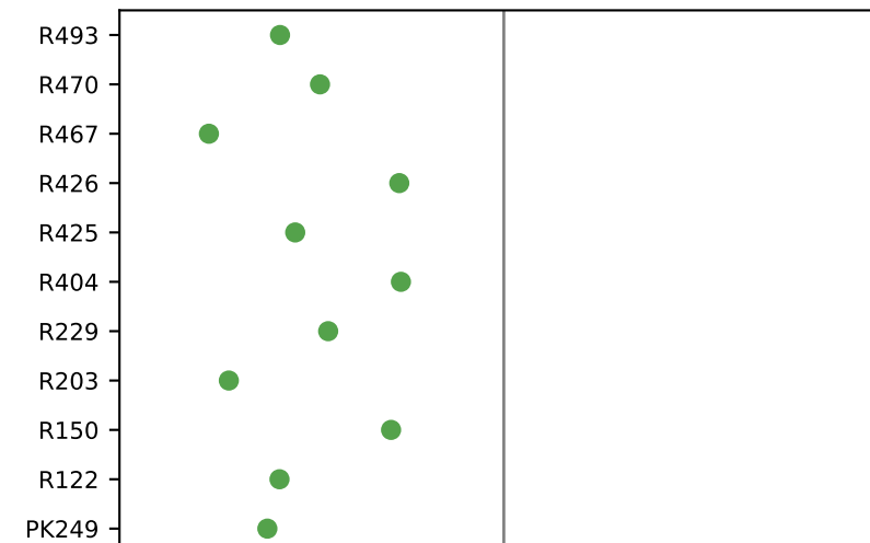
nearest distance
