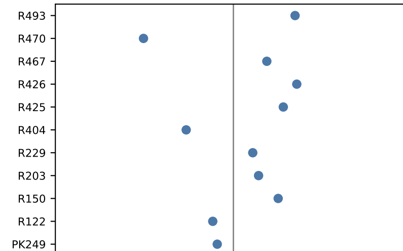
poincare radius
