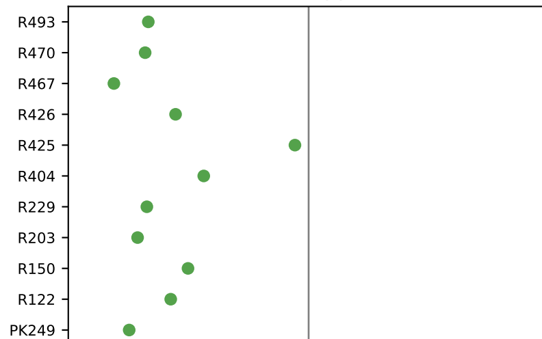
entropy
