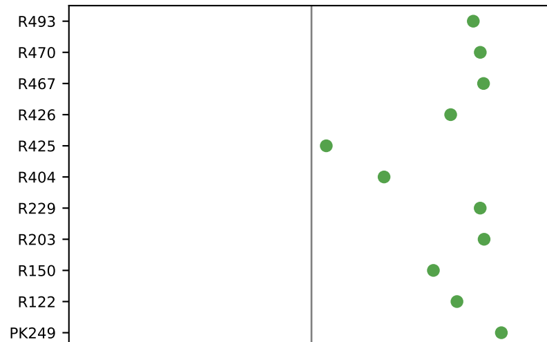
probability margin
