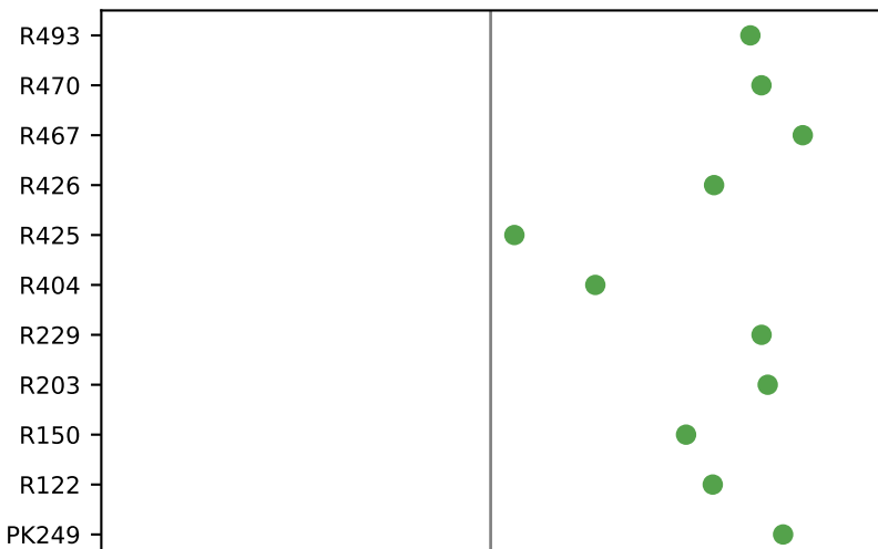
confidence
