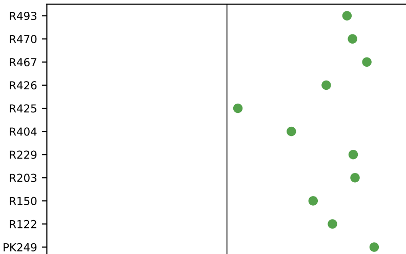
distance margin
