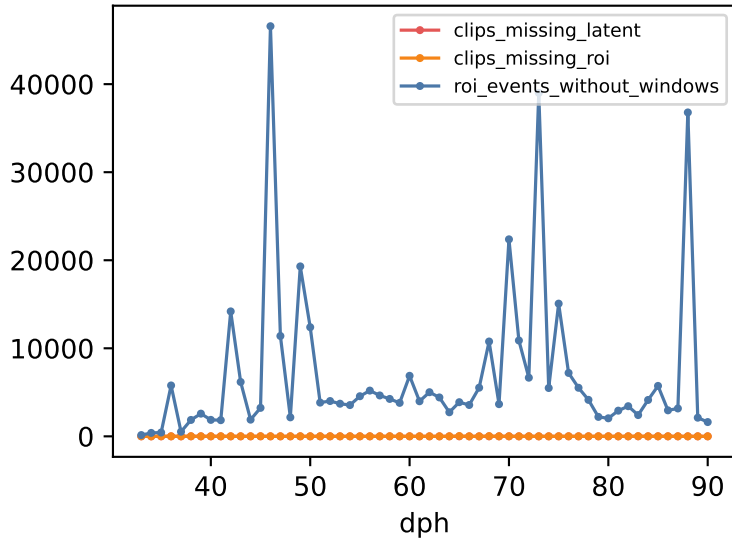
skip counts
