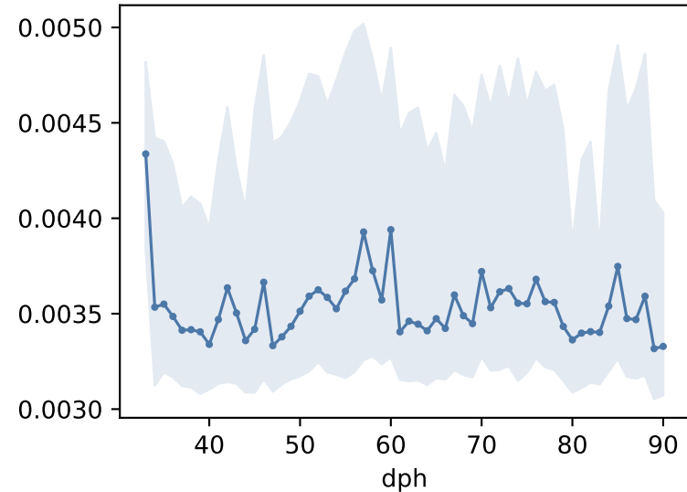
mean variance
