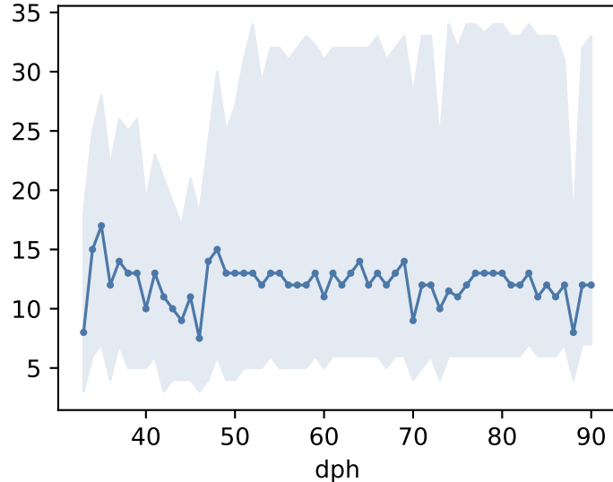
skip counts
