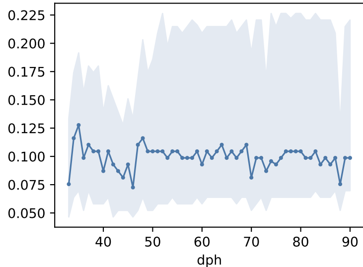
mean variance
