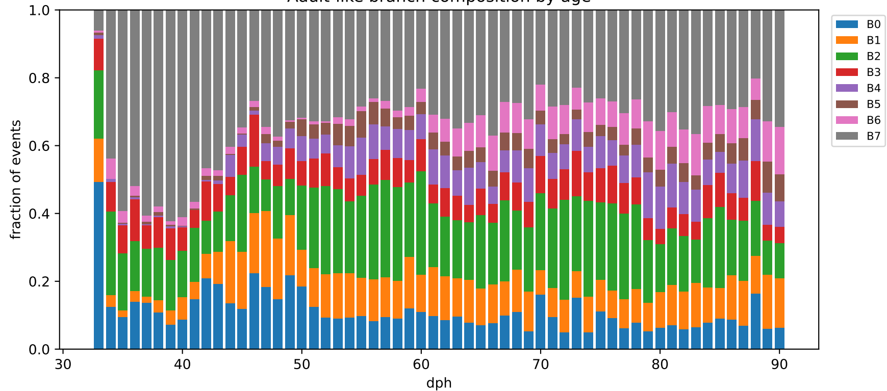
Adult-like branch composition by age
