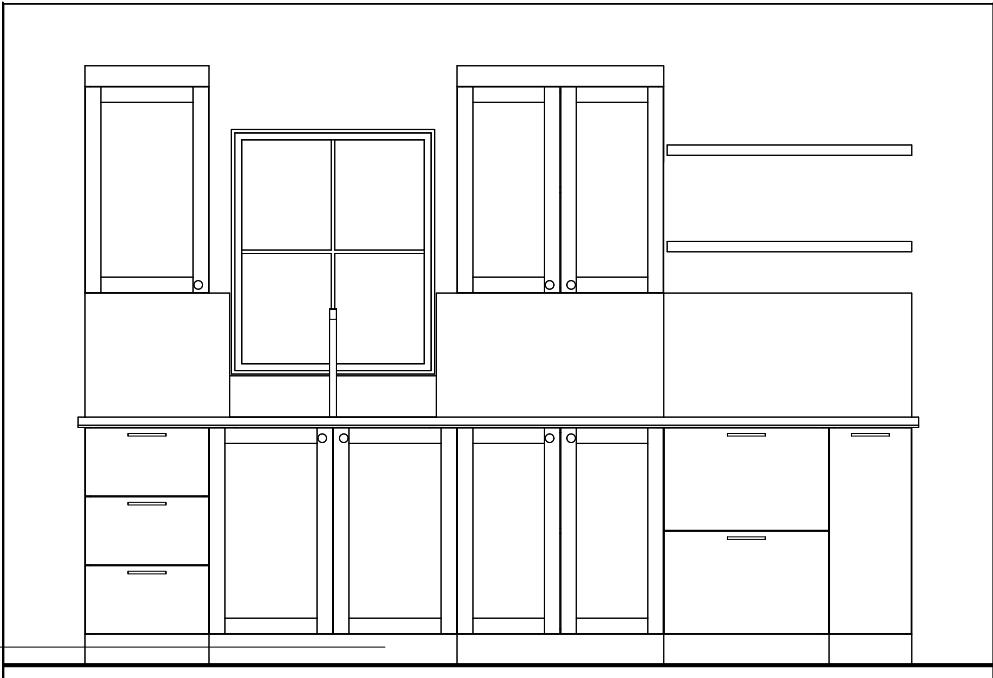
2 Cabinet Wall Elevation 1/2" = 1'-0"
