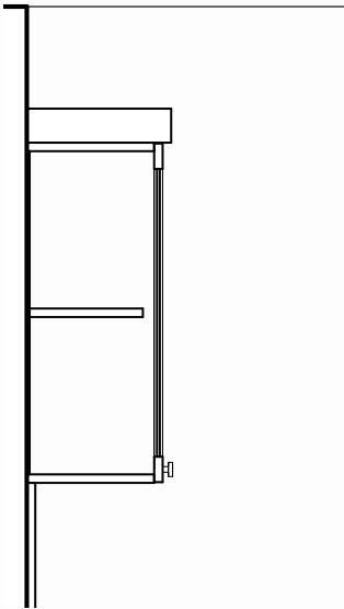
4 B30 Feature Cabinet - Section 3/4" = 1'-0"
