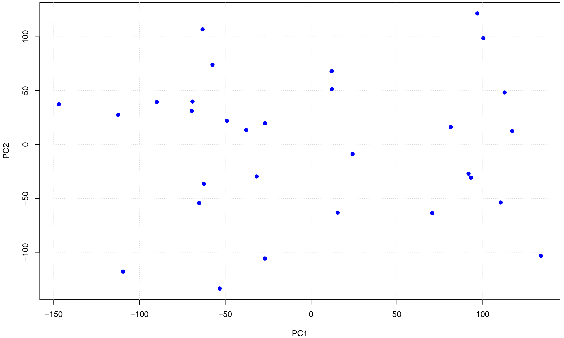
PCA of Normalized Expression Data
