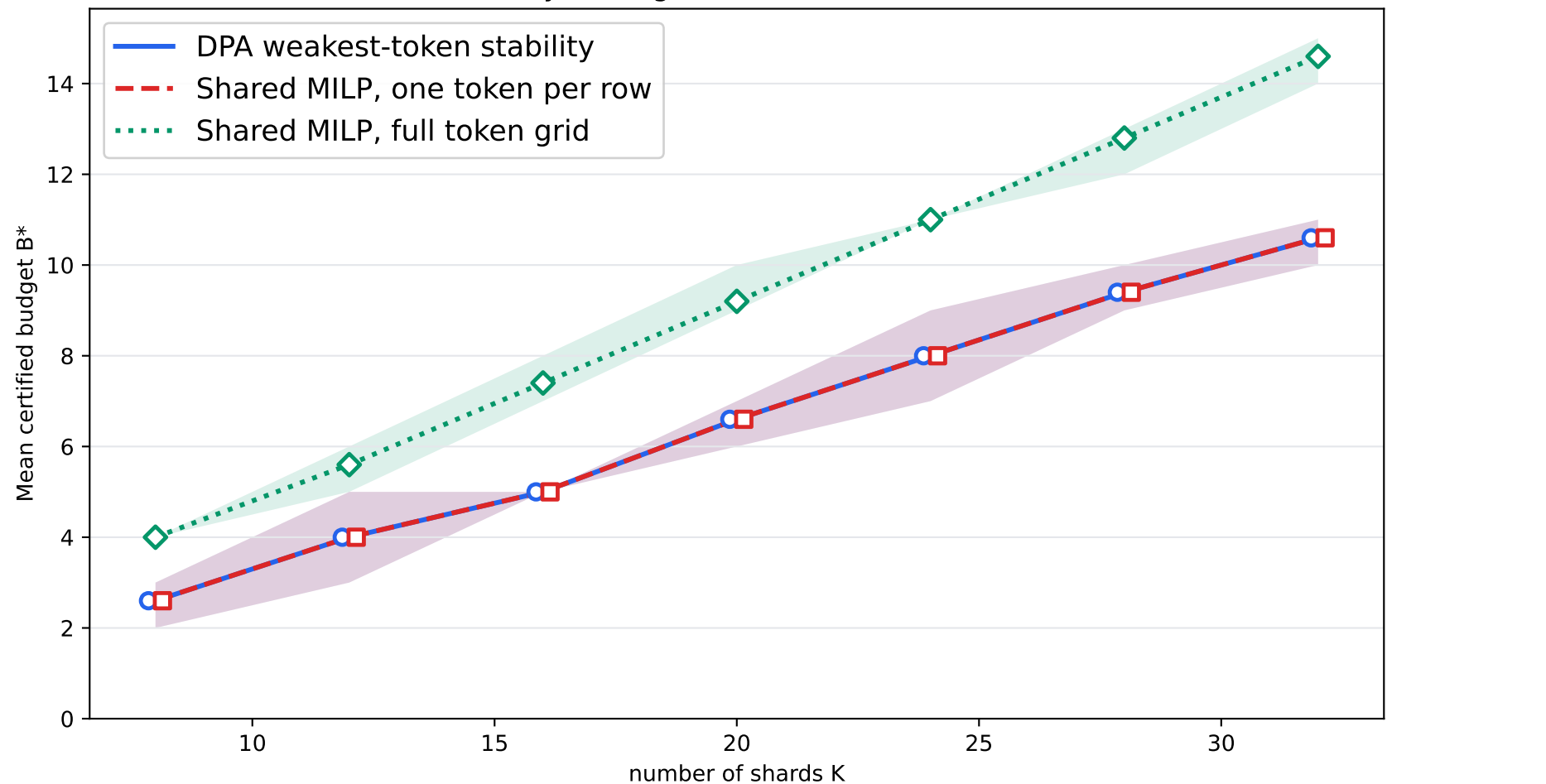
Stability scaling with number of shards K
