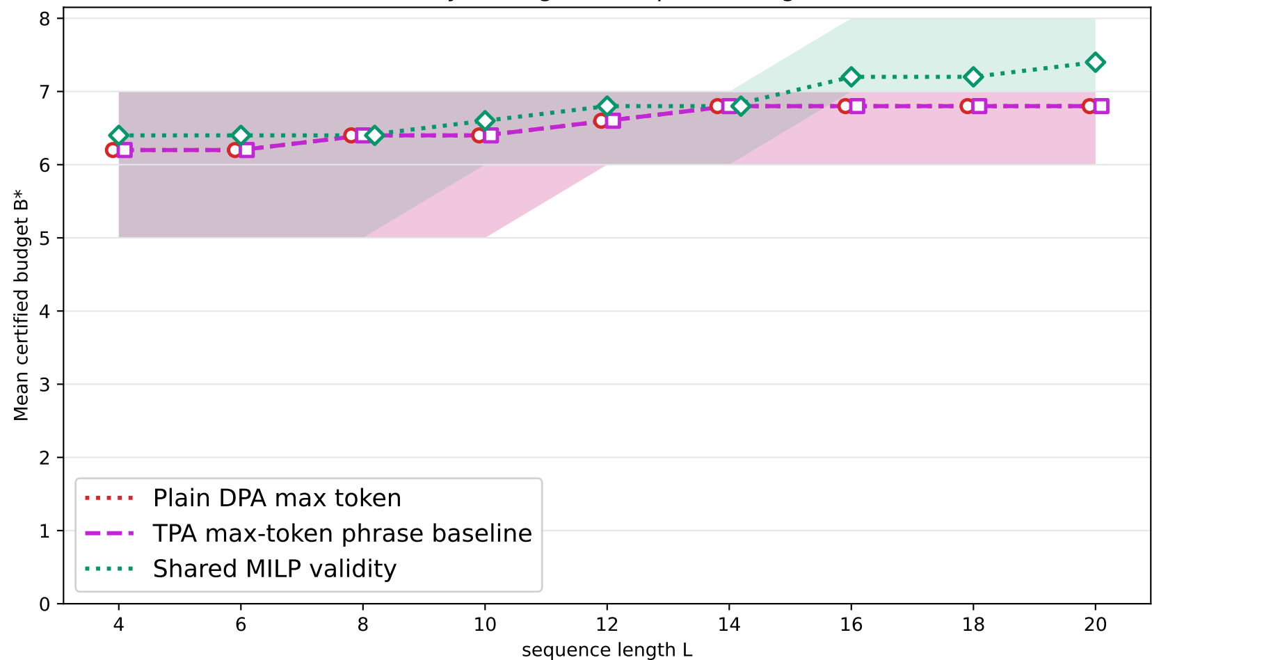
Validity scaling with sequence length L
