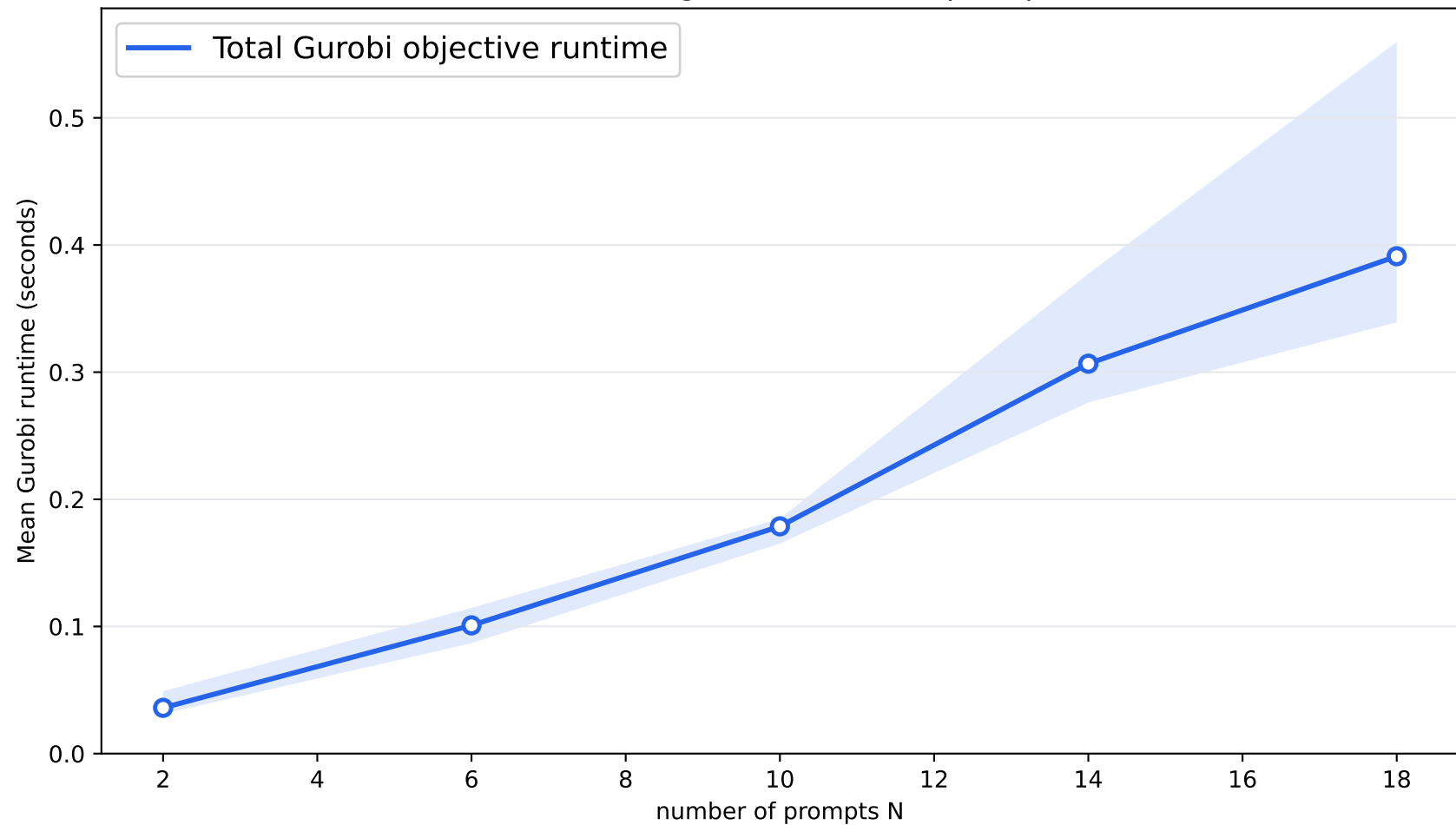
Runtime scaling with number of prompts N
