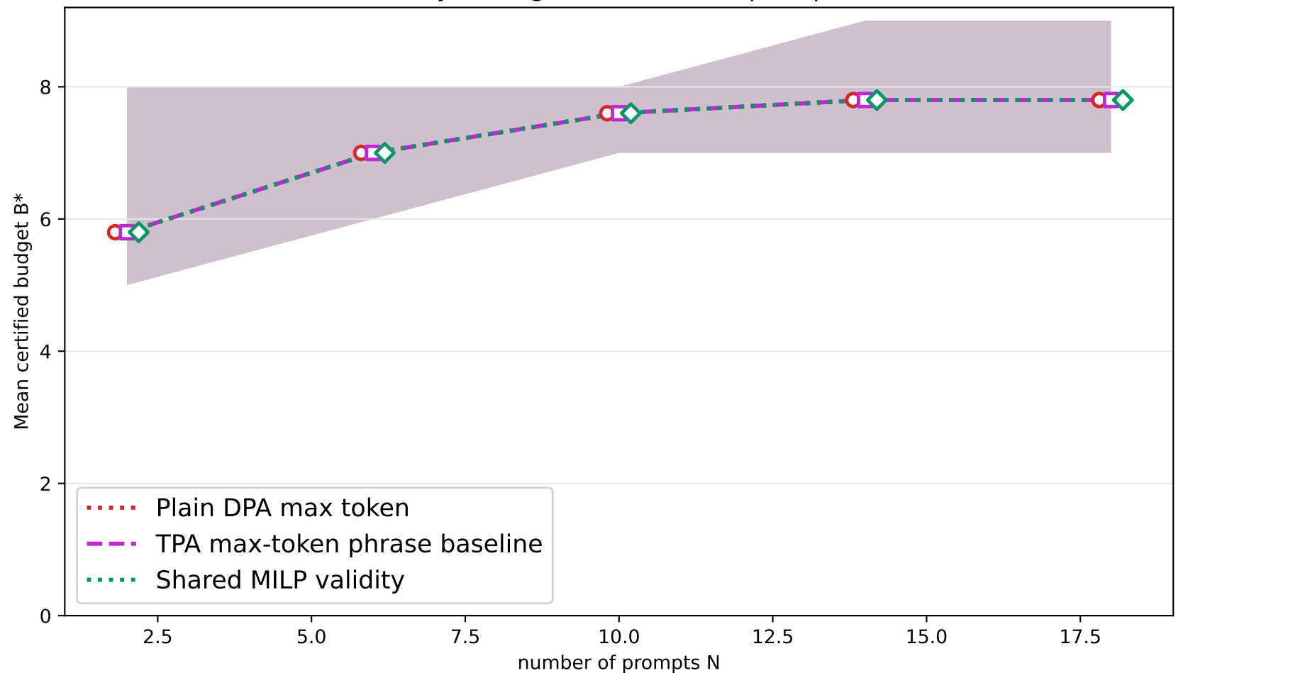
Validity scaling with number of prompts N
