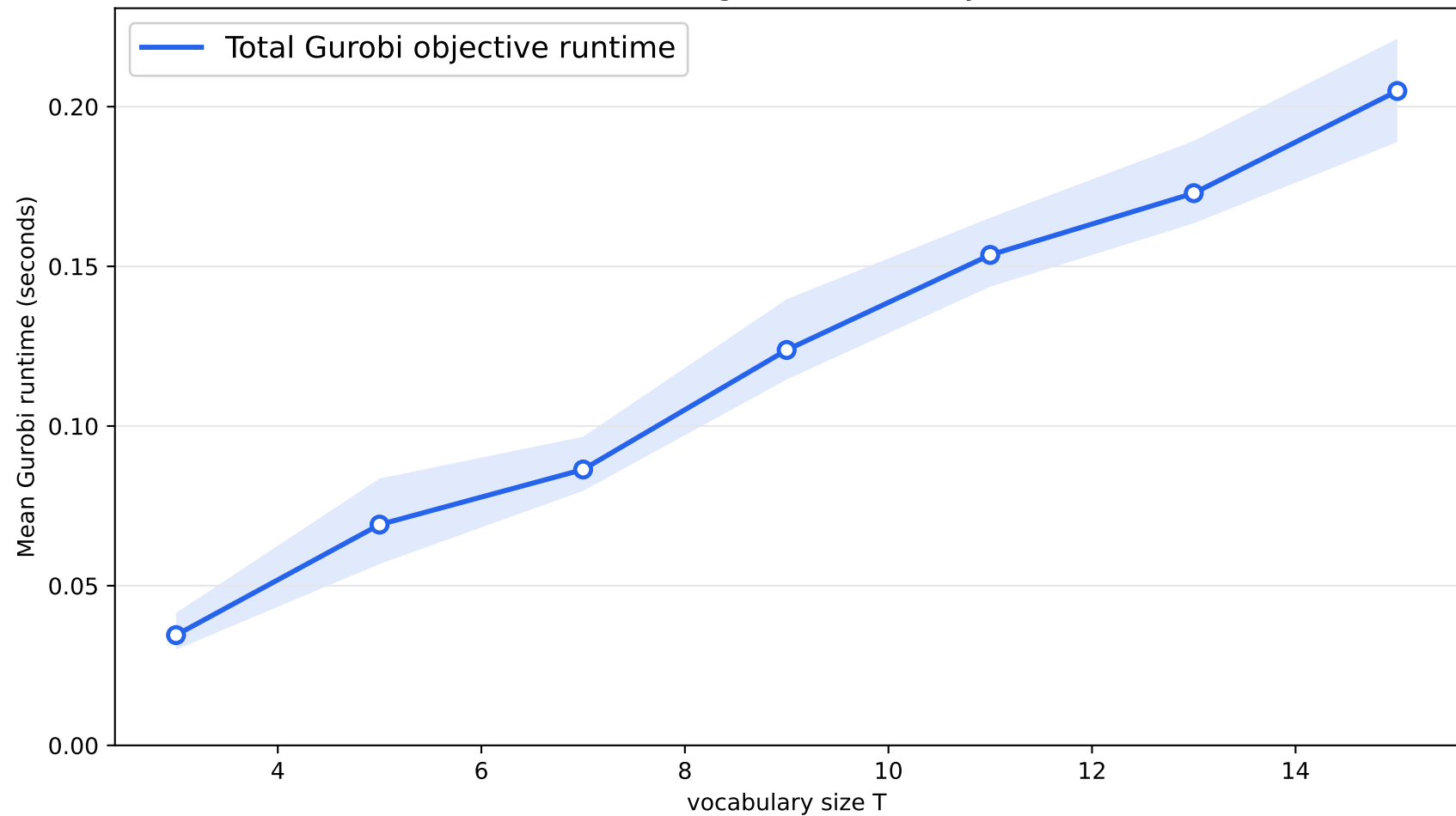
Runtime scaling with vocabulary size T
