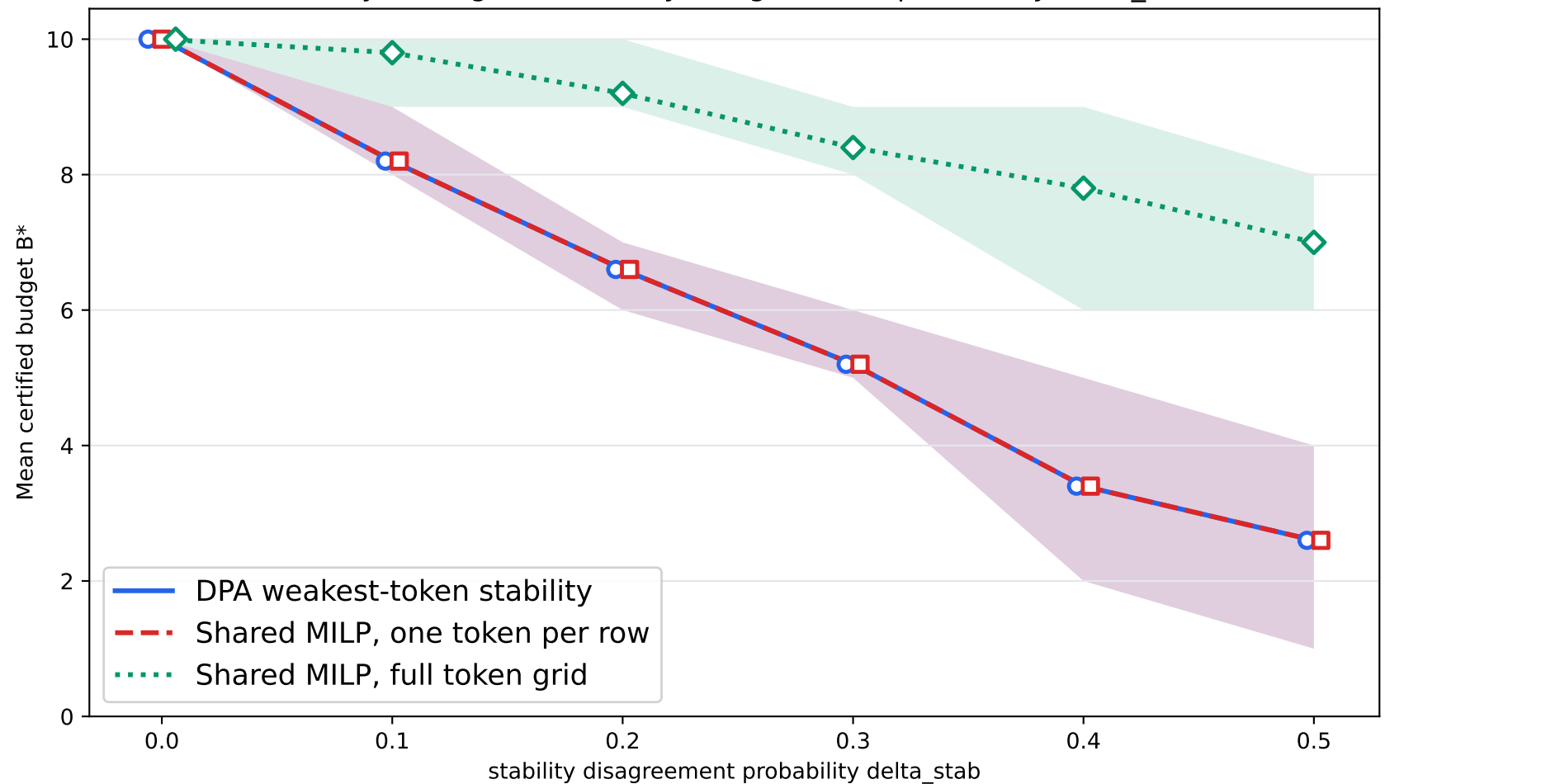
Stability scaling with stability disagreement probability \delta_{\text{stab}}
