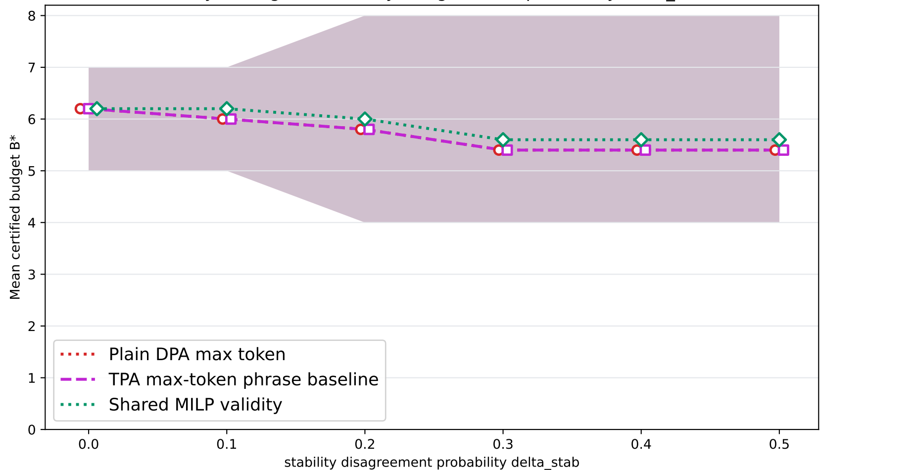
Validity scaling with stability disagreement probability \delta_{stab}
