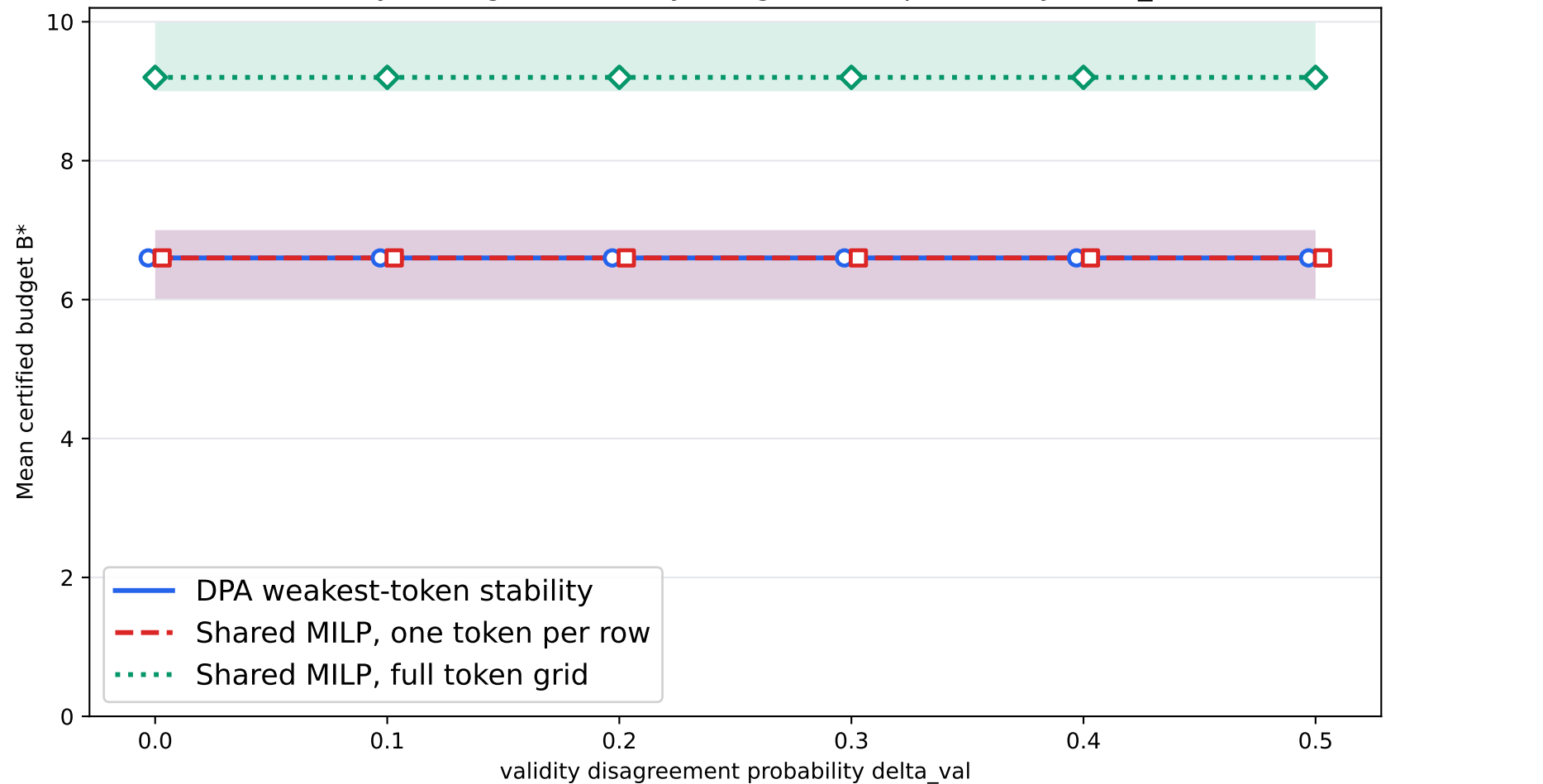
Stability scaling with validity disagreement probability \delta_{val}
