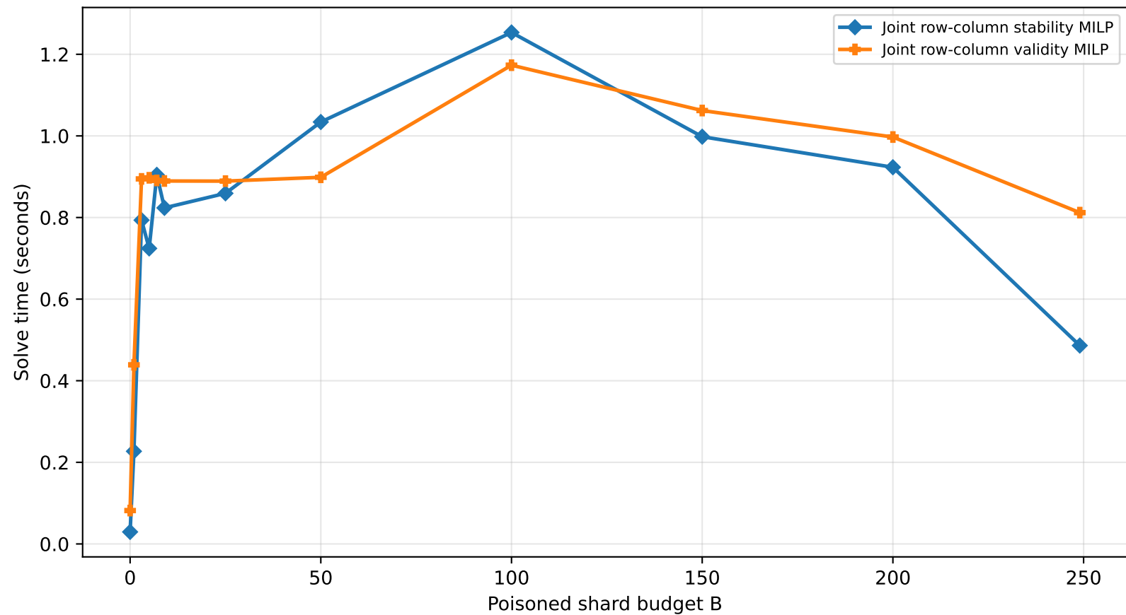
Full-scale certification MILP solve time
