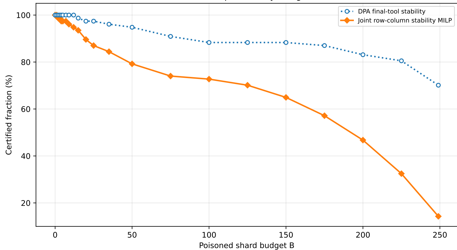
1B full H=20 top3 stability budget curve
