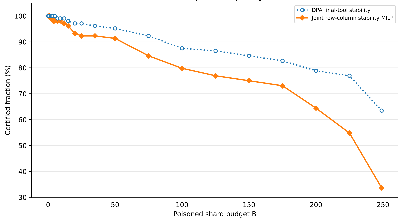
1B full H=15 top3 stability budget curve
