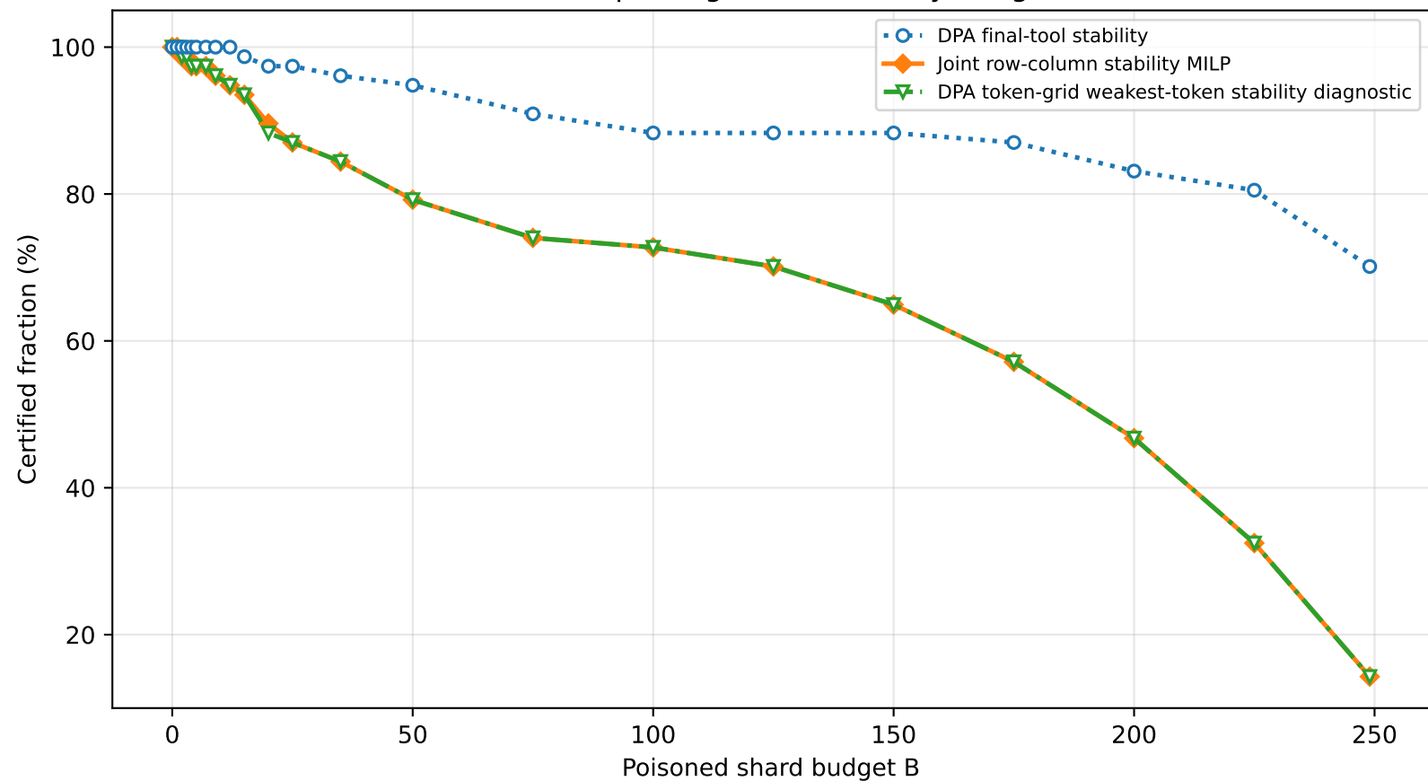
1B full H=20 top3 diagnostics stability budget curve
