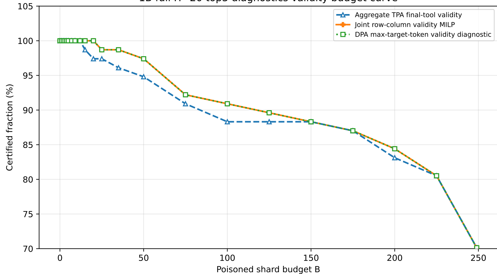
1B full H=20 top3 diagnostics validity budget curve
