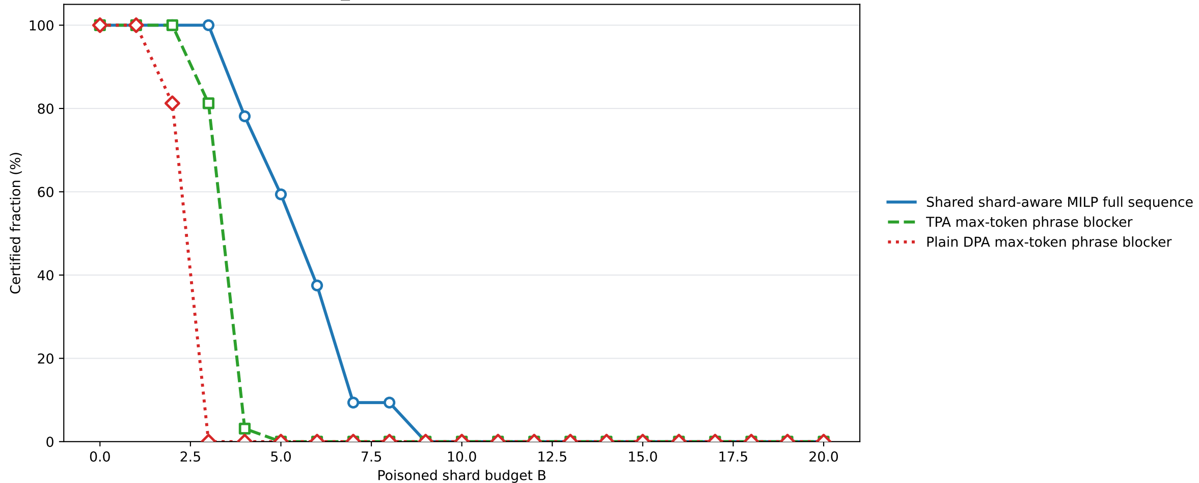
validity_demo certified fraction by budget
