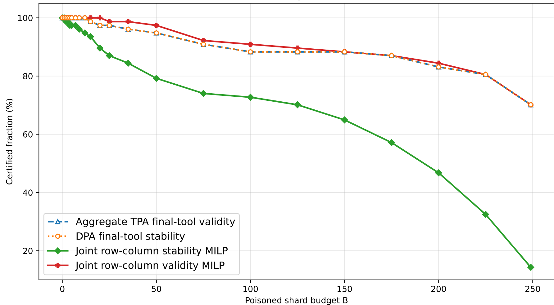
1B full H=20 top1 all methods
