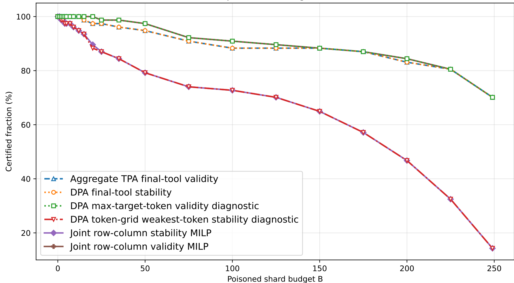
1B full H=20 top3 with DPA diagnostics all methods
