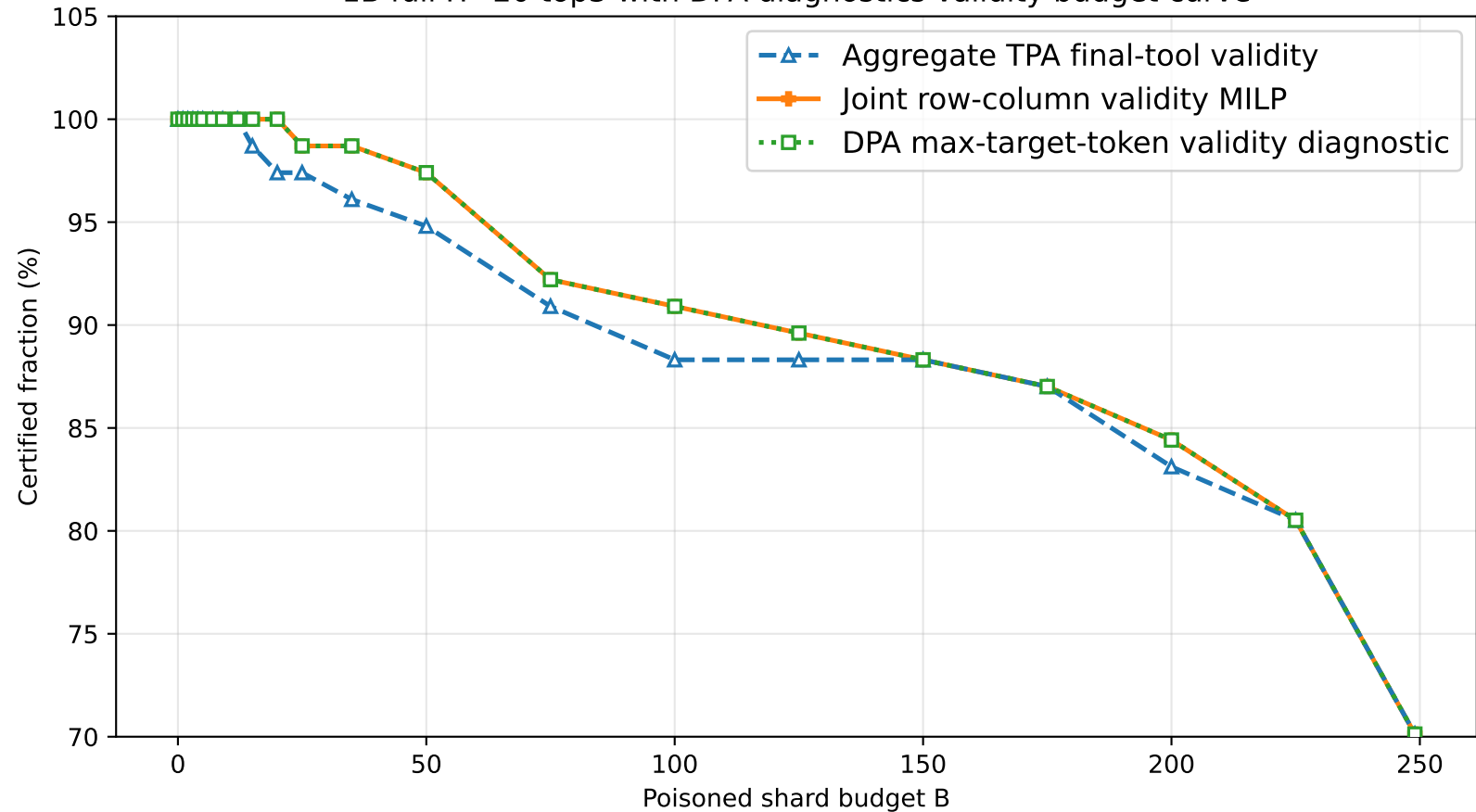
1B full H=20 top3 with DPA diagnostics validity budget curve
