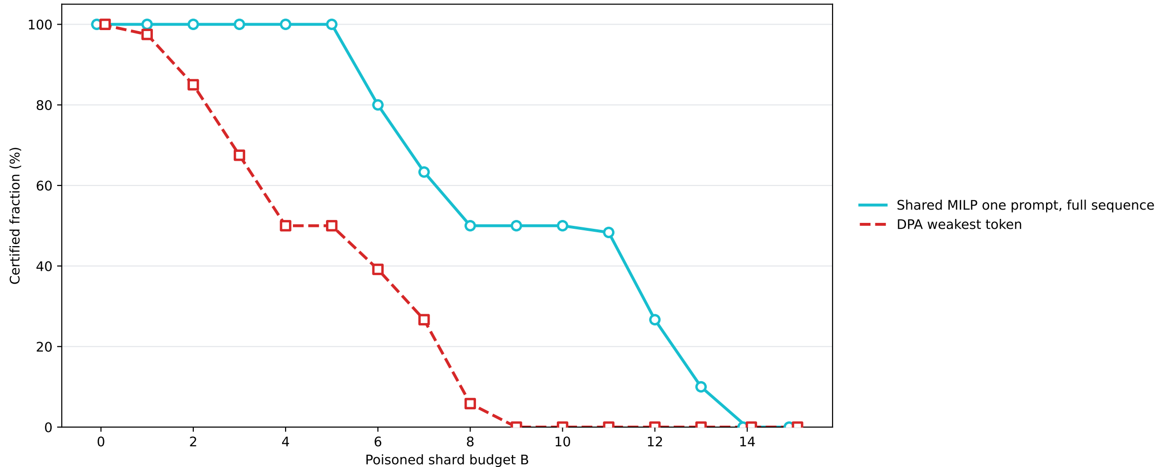
Stability one prompt budget curve
