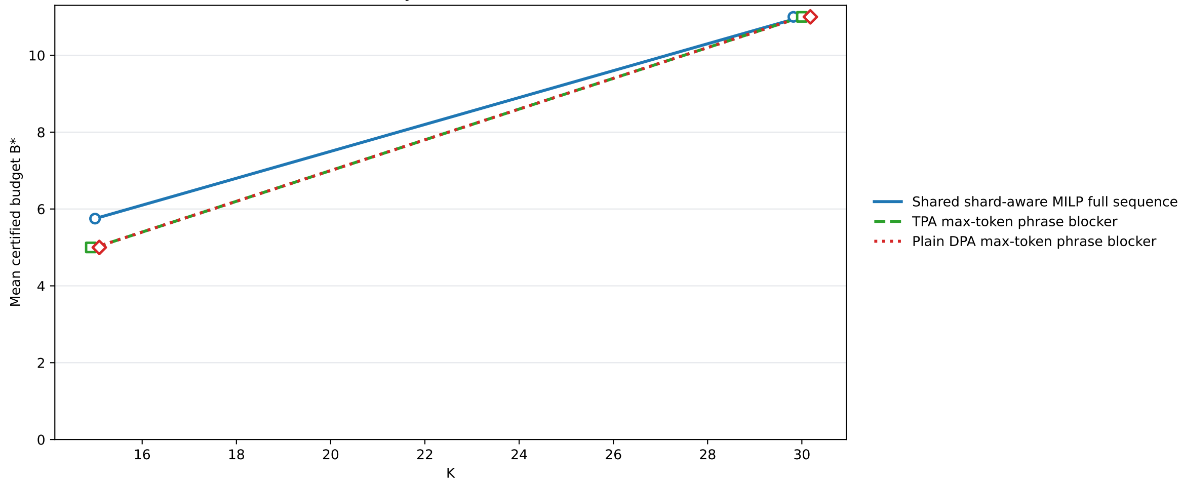
Validity certificate vs K
