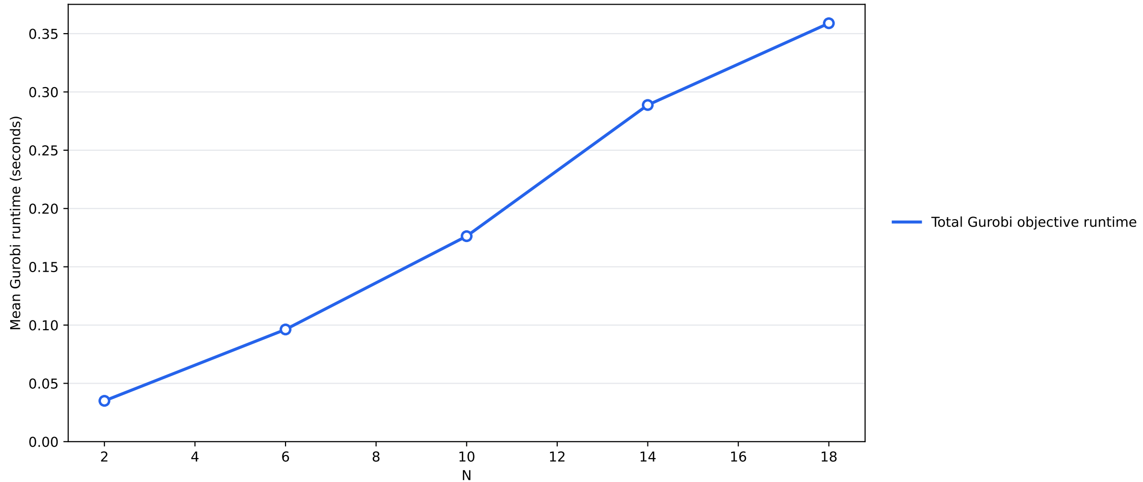
Runtime scaling with N
