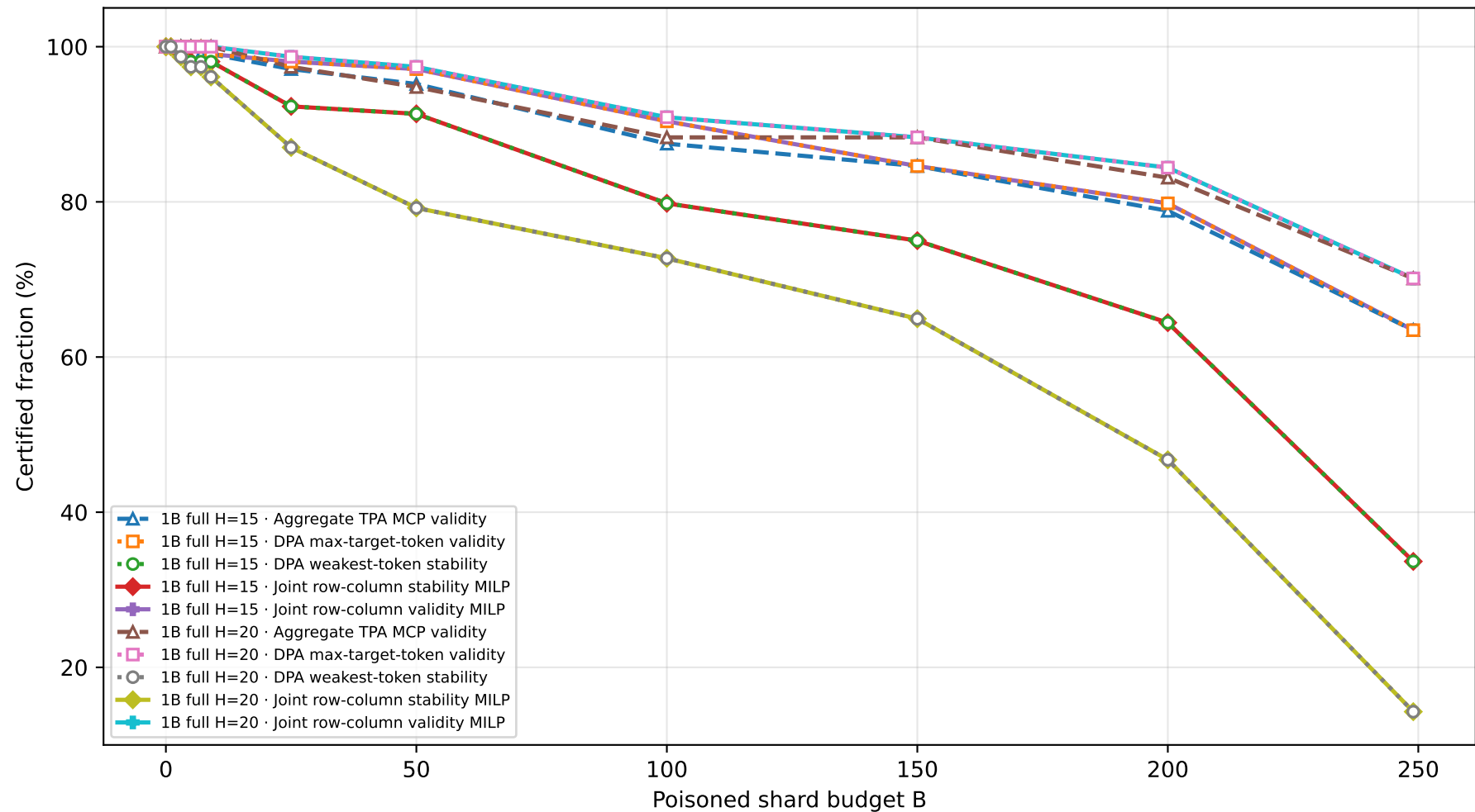
Full-scale certification all methods
