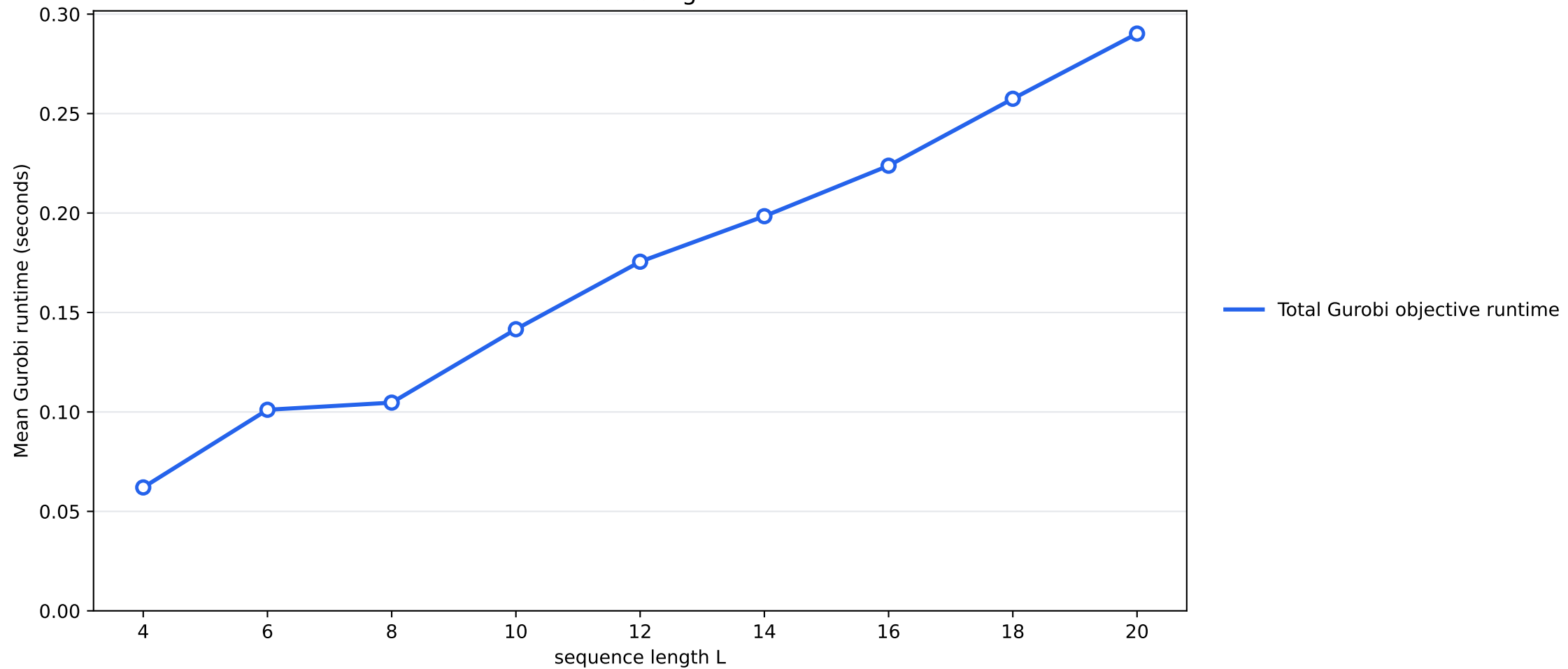
Runtime scaling with L
