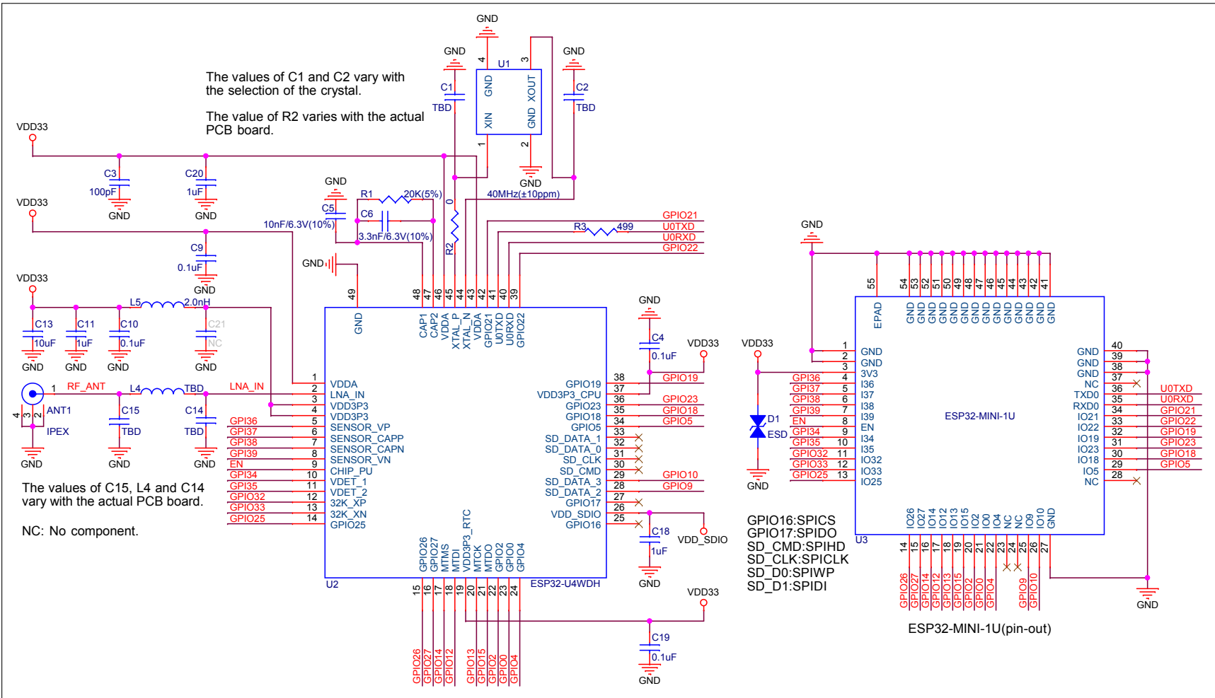
Figure 8: ESP32-MINI-1U Schematics
