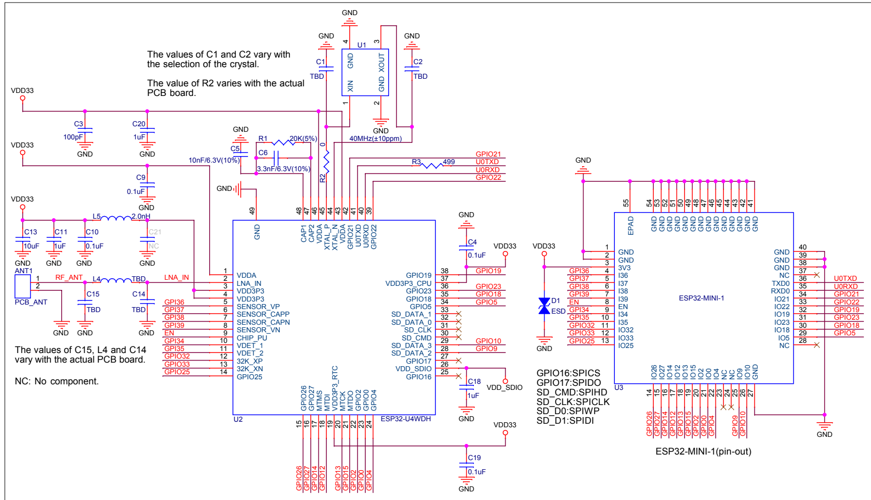
Figure 7: ESP32-MINI-1 Schematics
