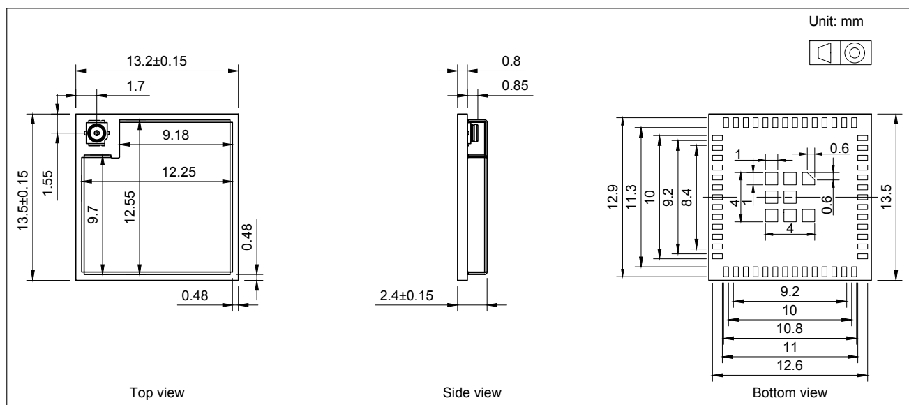
Figure 11: ESP32-MINI-1U Physical Dimensions
