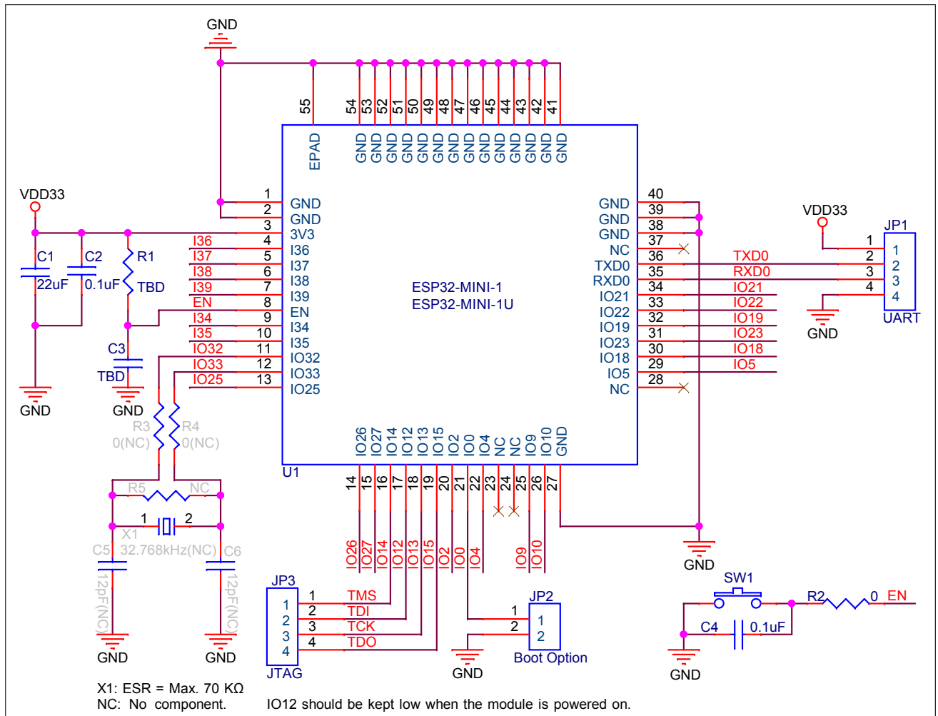
Figure 9: Peripheral Schematics
