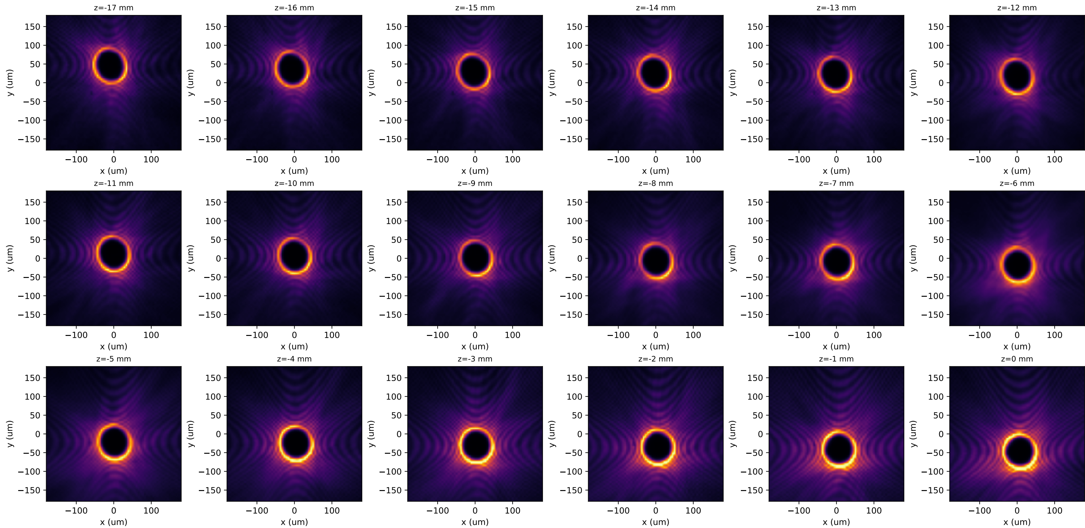
Measured q=20 BMG stack — fixed camera coordinates, four repeats averaged per z
