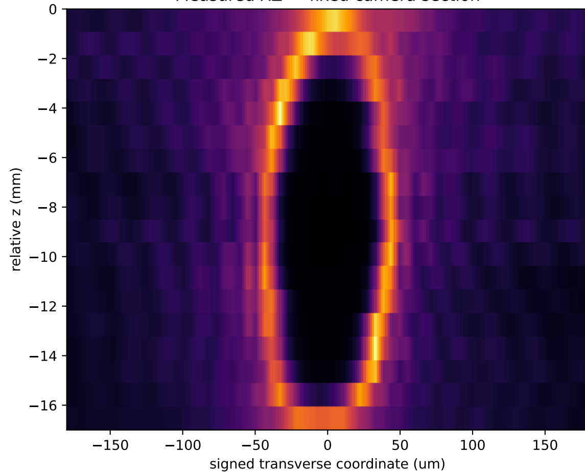
Measured XZ — fixed camera section
