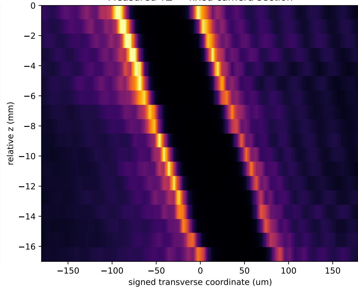
Measured YZ — fixed camera section
