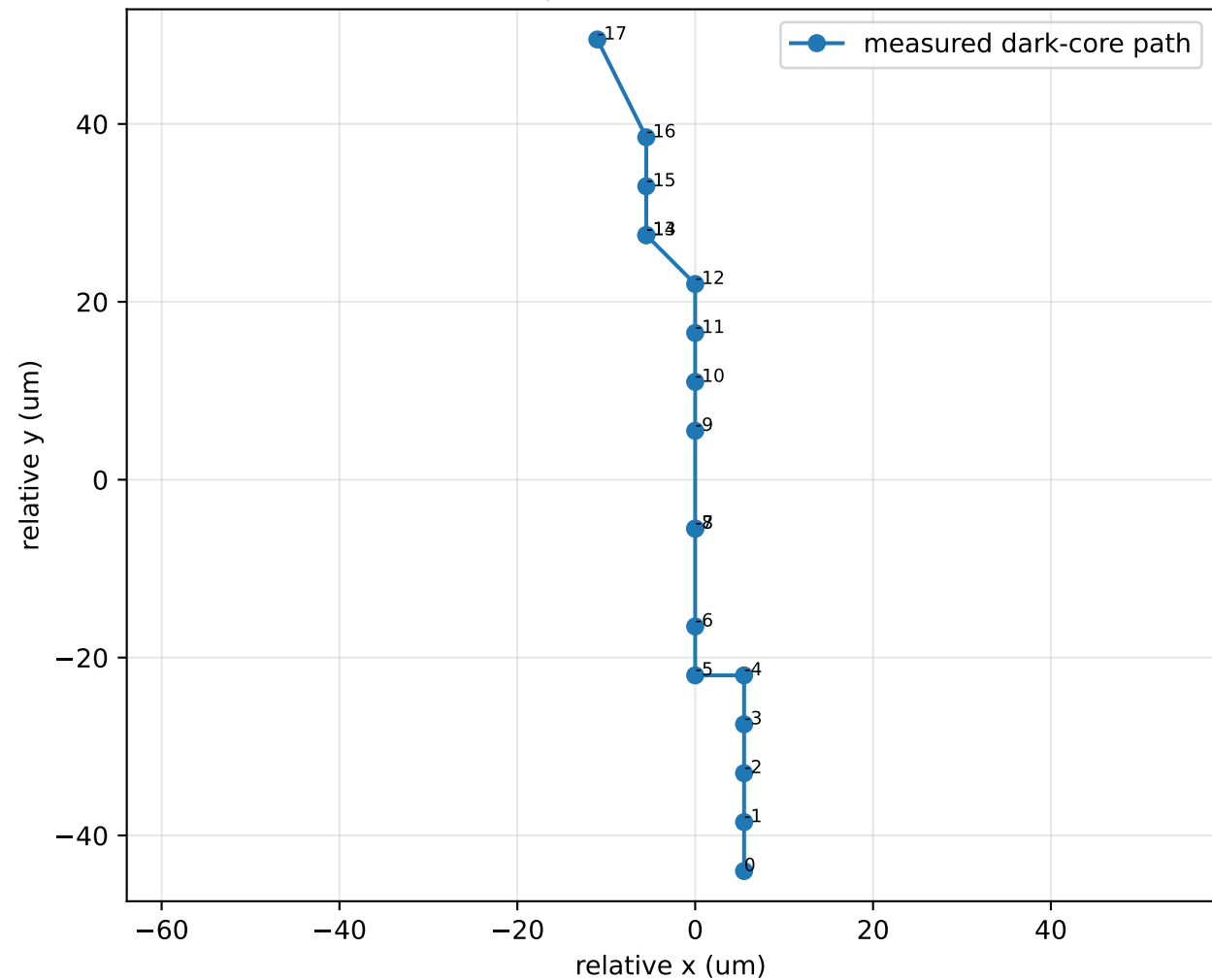
Measured beam path in fixed camera coordinates
