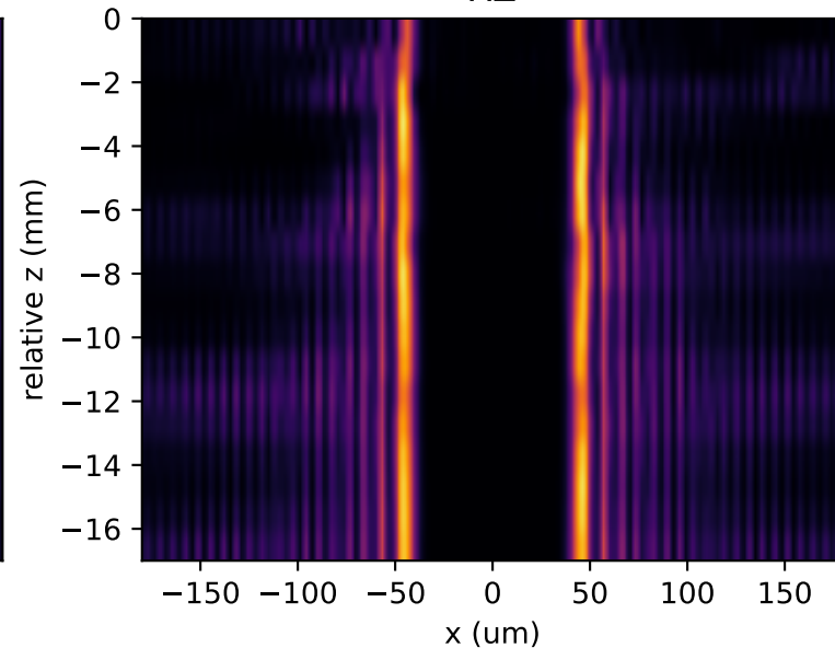
horizontal section
