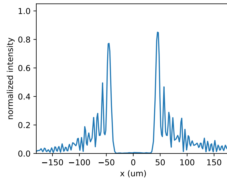
horizontal section
