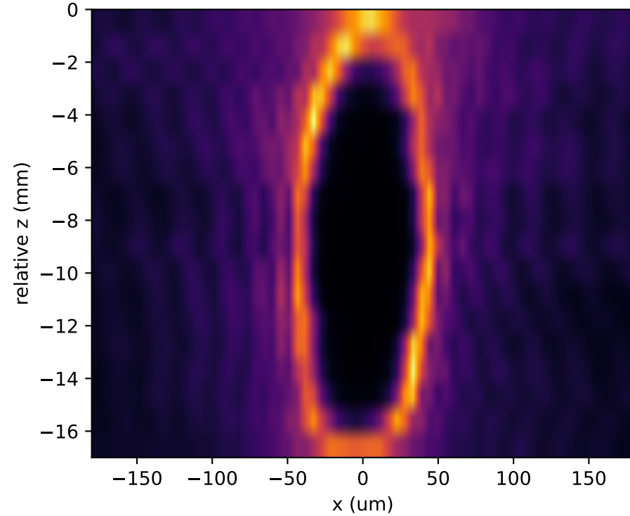
Measured fixed-camera XZ
