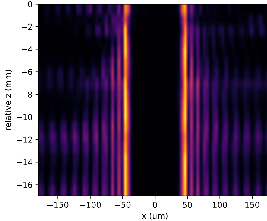
Nominal-model XZ
