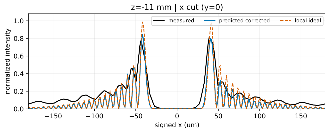
Measured / predicted-corrected / local-ideal linear sections
