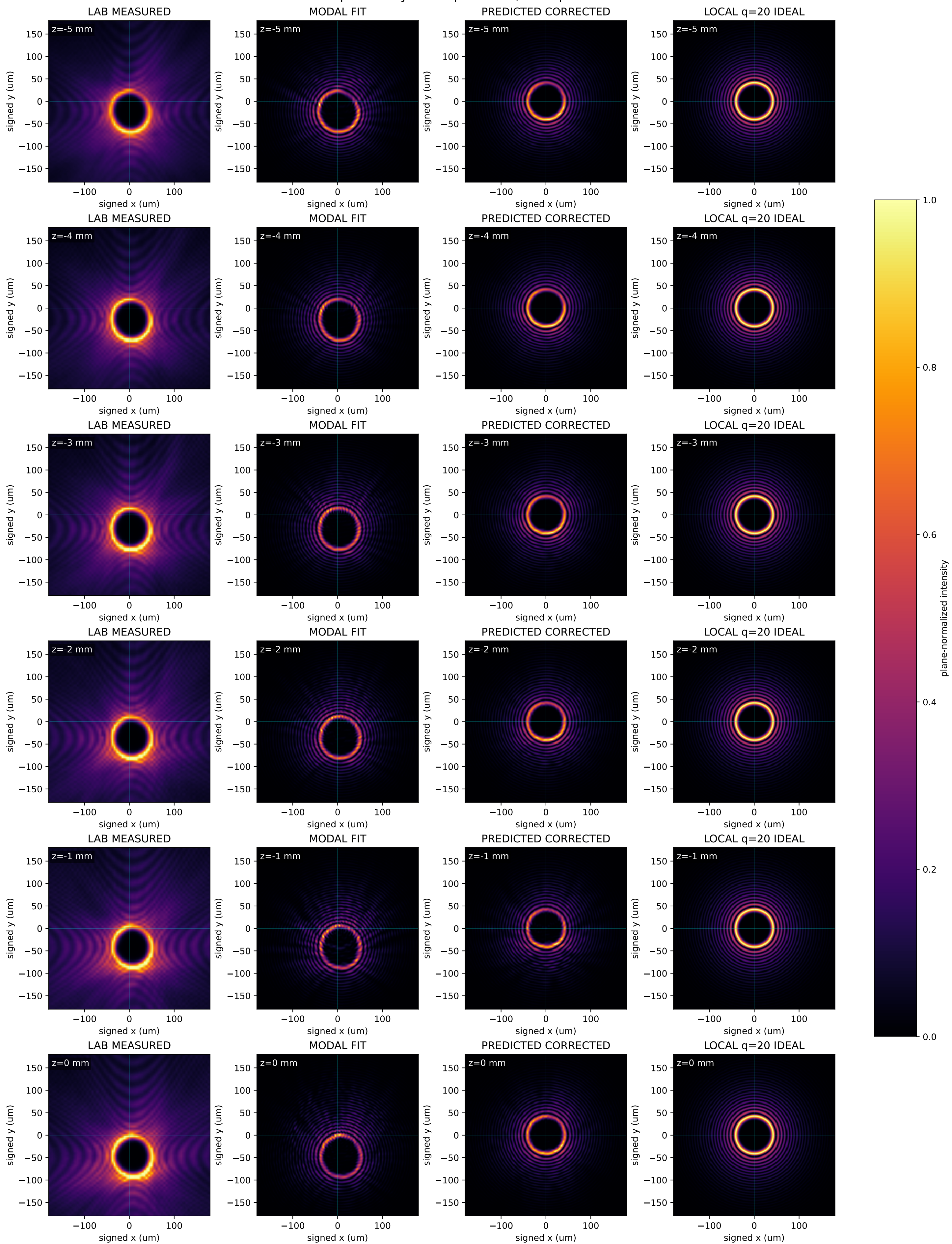
Global-branch q=20 retrieval: measured, fit, predicted correction, and local ideal corrected is a phase-only model prediction, not a post-SLM measurement
