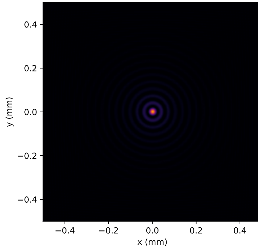
after candidate | z=120.0 mm
