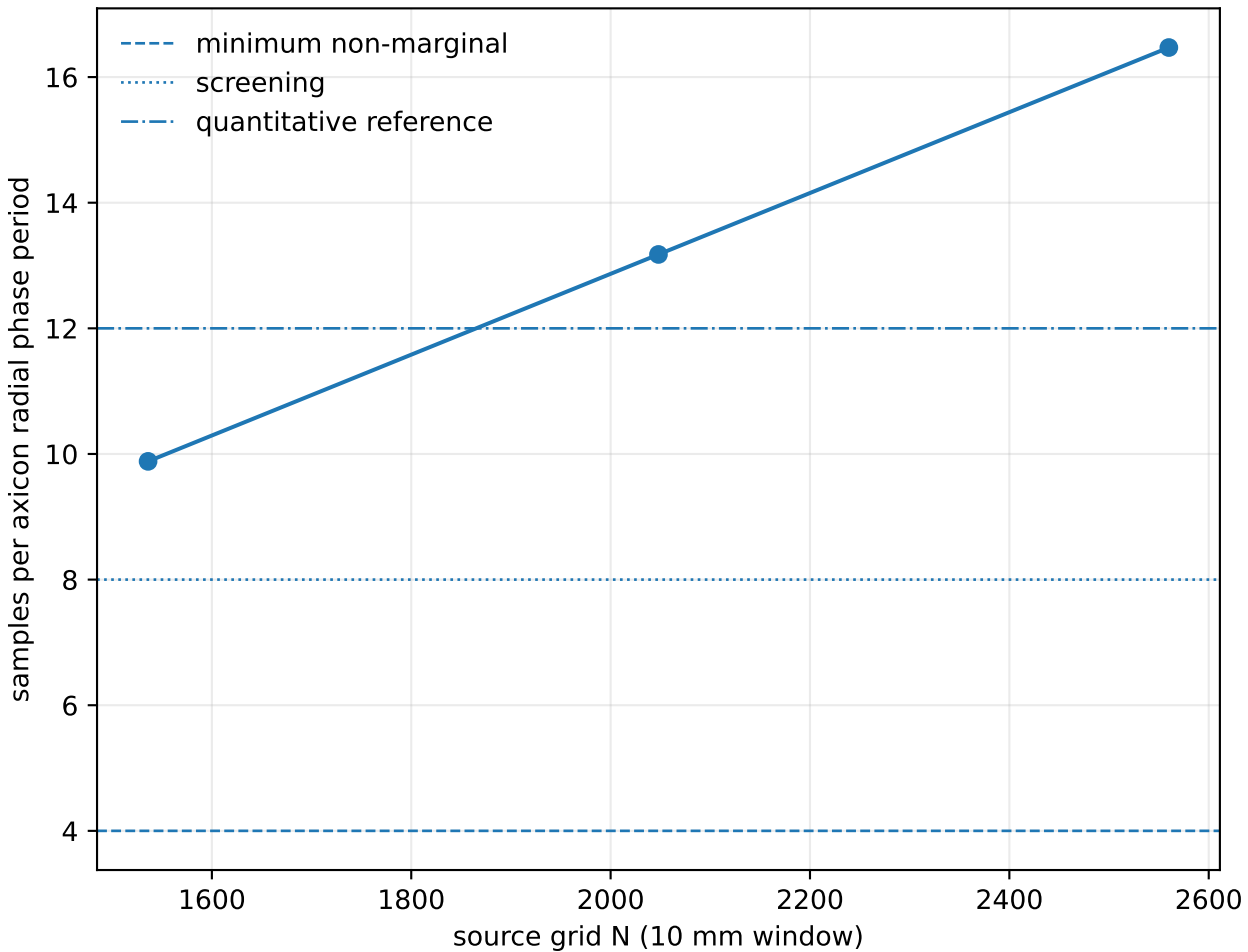
Source-plane axicon sampling
