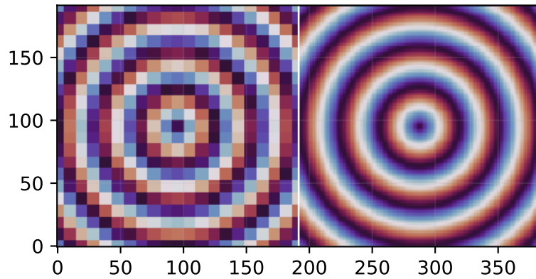
wrapped axicon phase | N512 left, N3072 right
