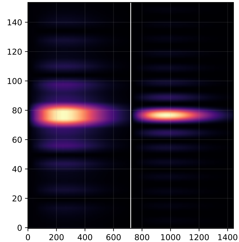
N512 left versus N3072 right | matched detail
