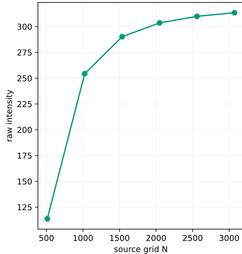
B0 raw on-axis intensity at z=60 mm
