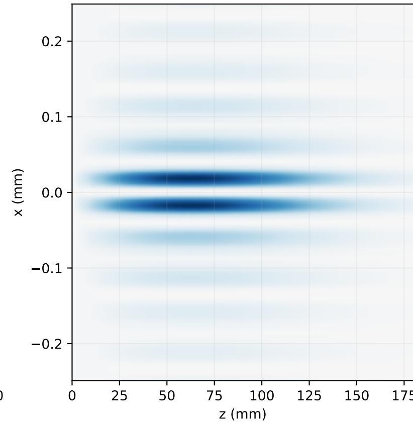
N3072 - interpolated N512
