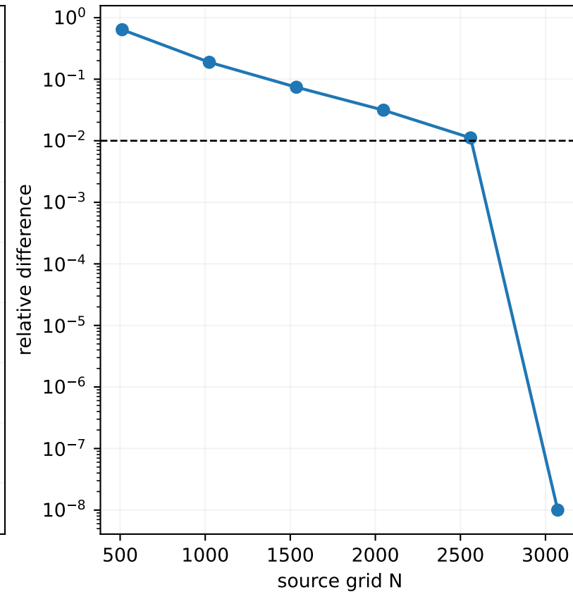
relative difference to N3072
