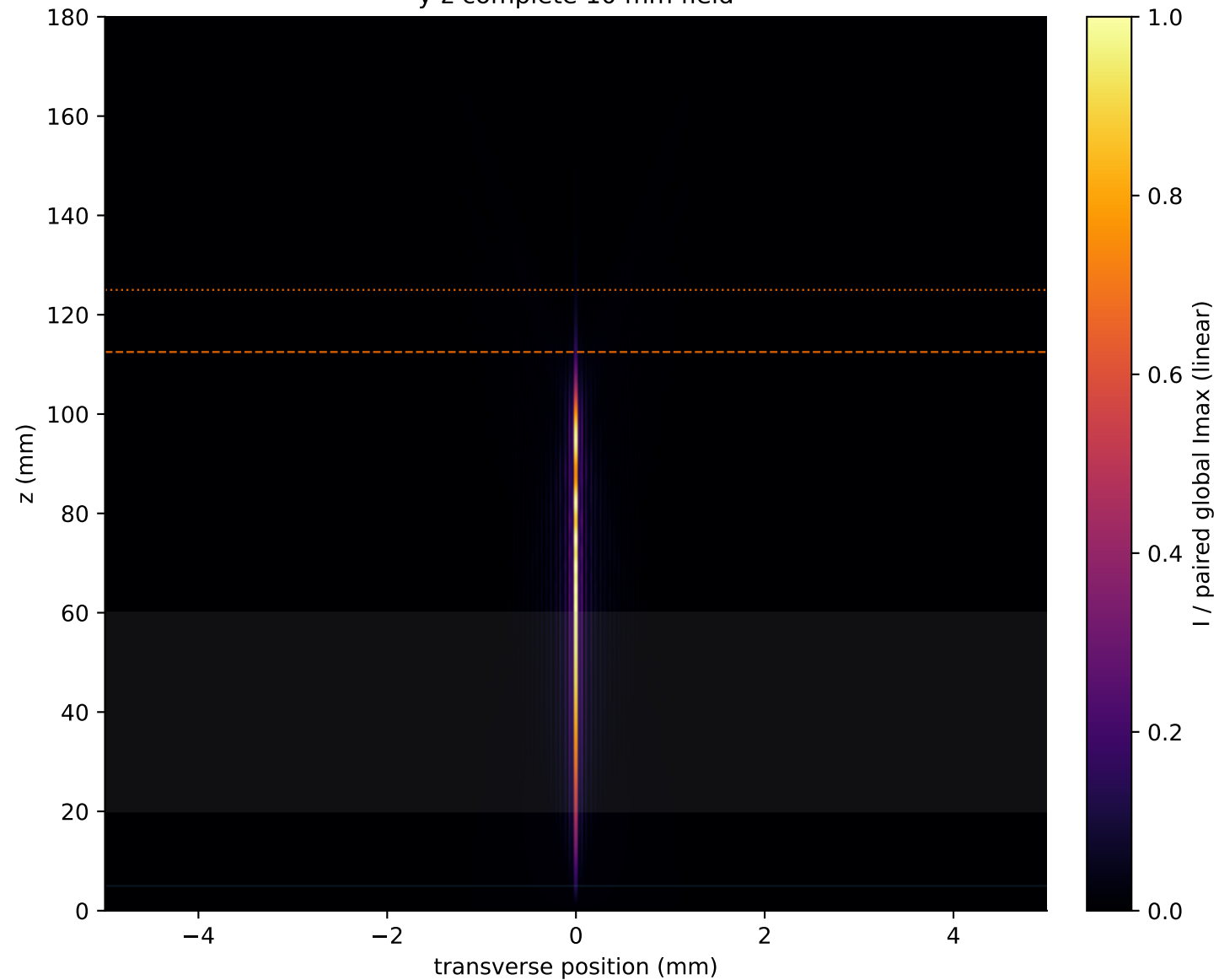
y-z complete 10 mm field
